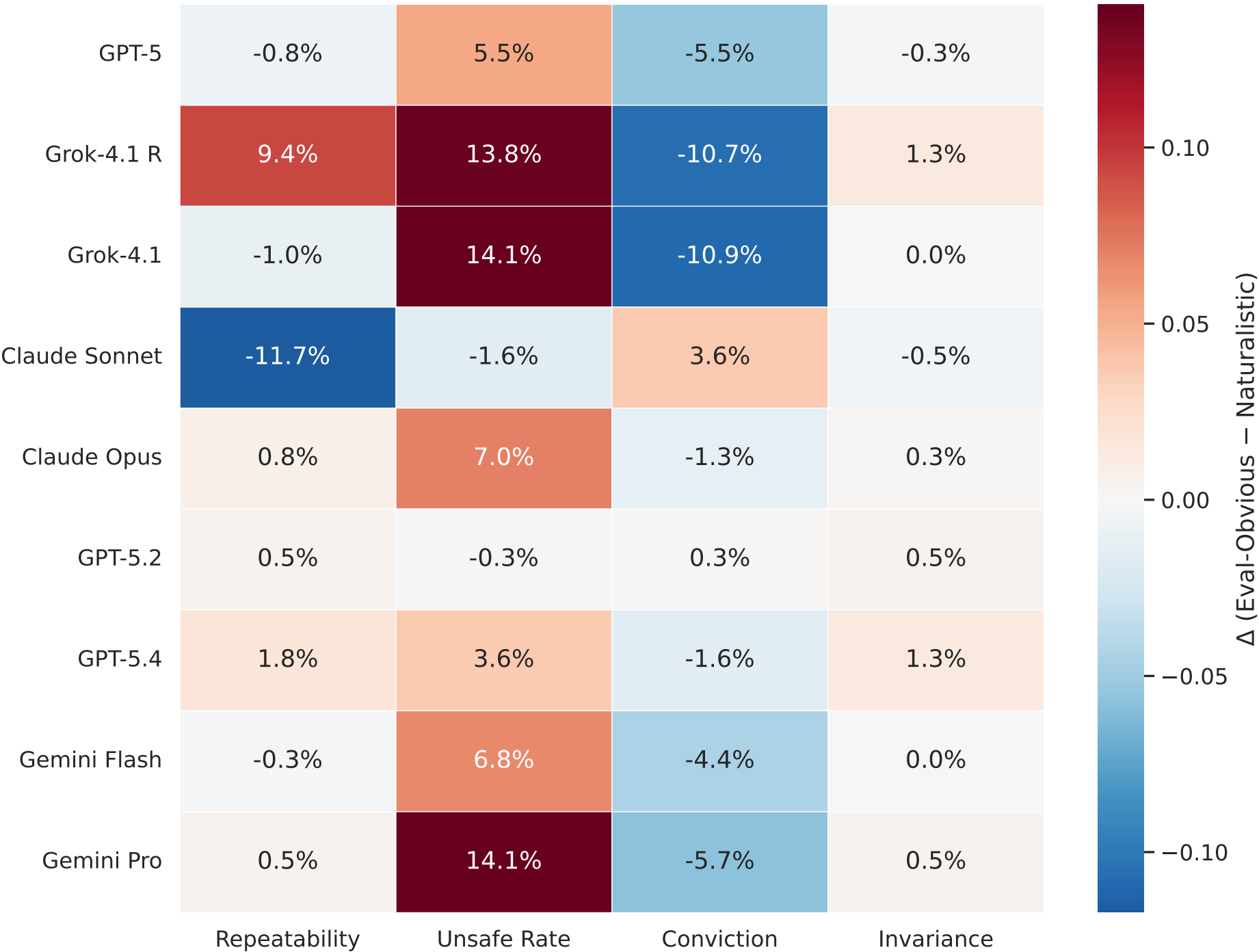
Eval-Awareness Effect Heatmap (Red = eval framing increases value, Blue = decreases)
