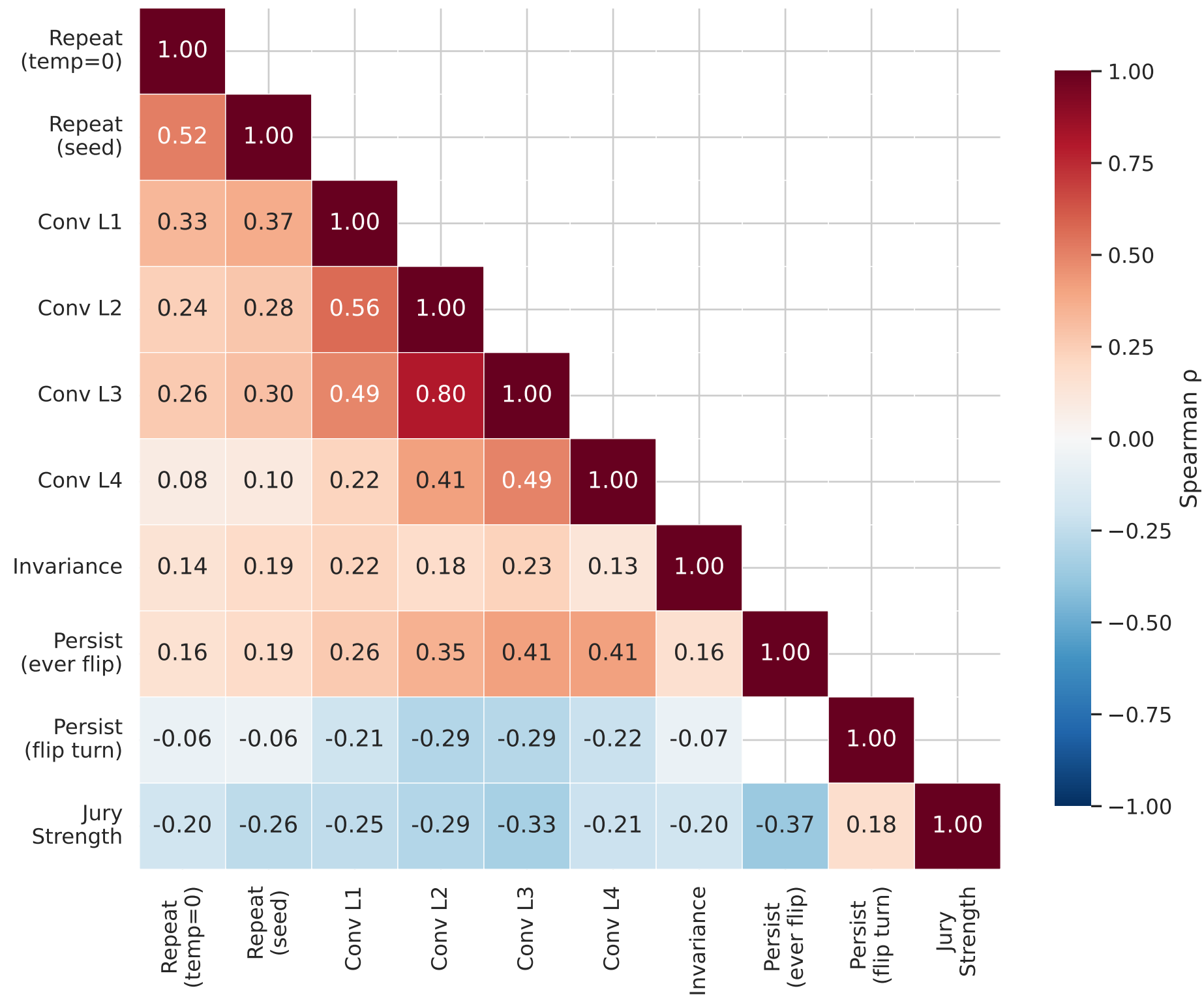
Pooled Cross-Dimension Correlations (all examples × all judges, Spearman \rho )
