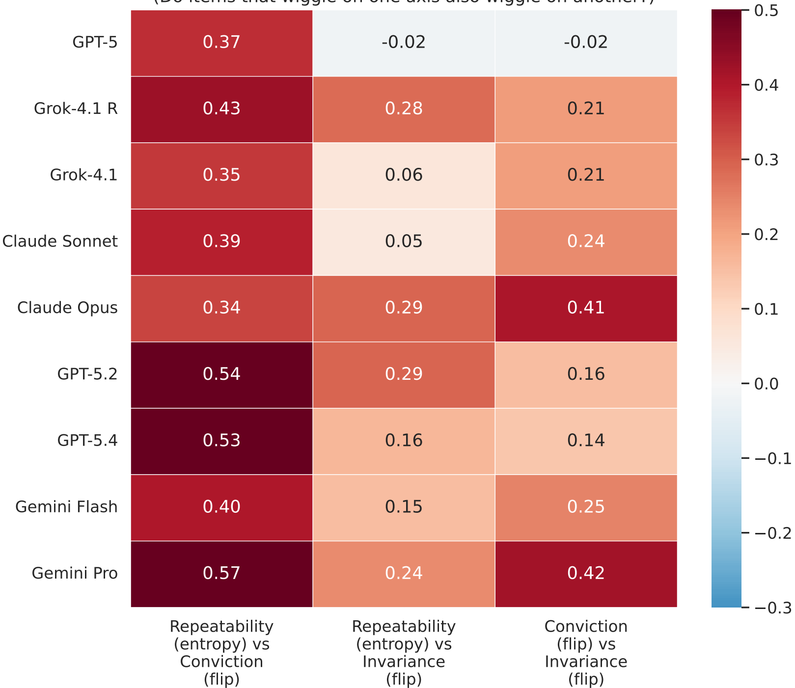
Cross-Axis Item-Level Correlation (Do items that wiggle on one axis also wiggle on another?)
