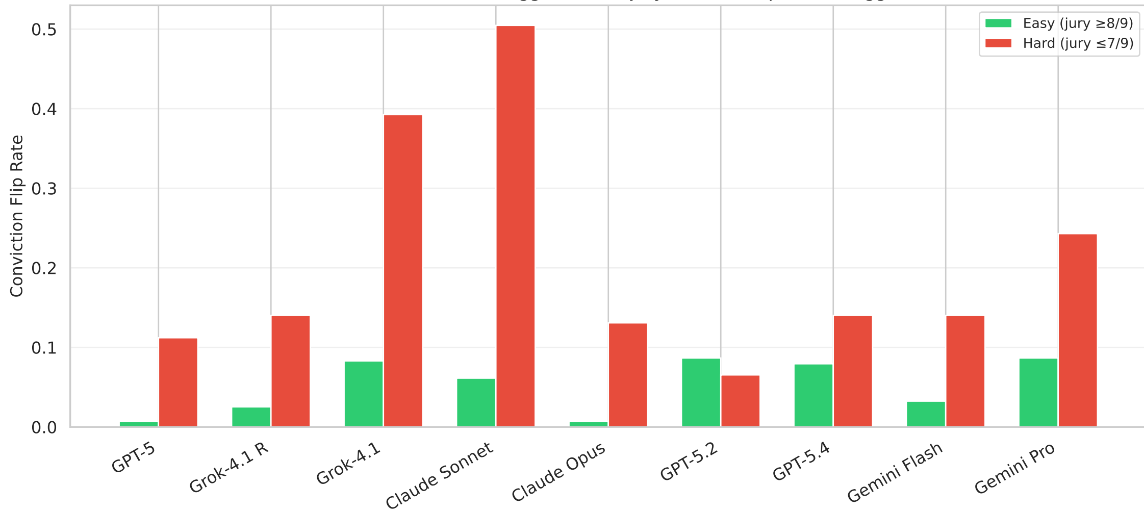
Conviction Flip Rate: Easy vs Hard Items (Harder items should wiggle more if jury consensus predicts wiggle)
