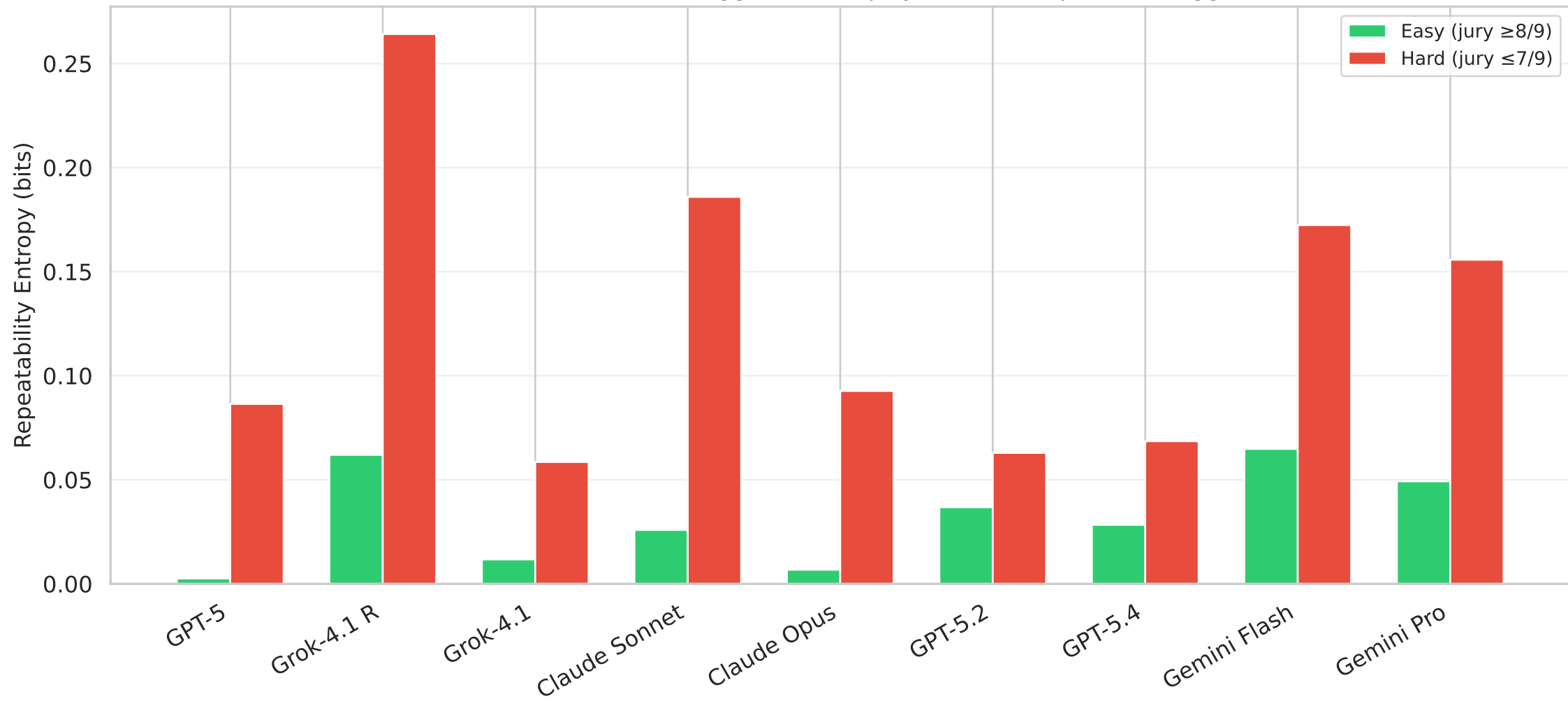
Repeatability Entropy (bits): Easy vs Hard Items (Harder items should wiggle more if jury consensus predicts wiggle)
