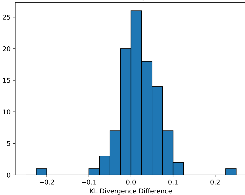
Distribution of KL Divergence Differences
