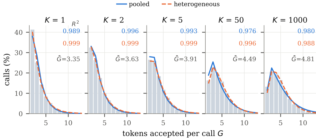
Figure 5: Committed tokens per call against ensemble width. Bars are observed; lines are the branching model equation 7 with a single (\pi_0, p, \rho) shared across all five panels ( pooled ) and with p integrated over a fitted \text{Beta}(a, b) population ( heterogeneous ). R^2 per curve is printed in the curve’s own colour. One three-parameter model tracks the distribution over three orders of magnitude of K .
