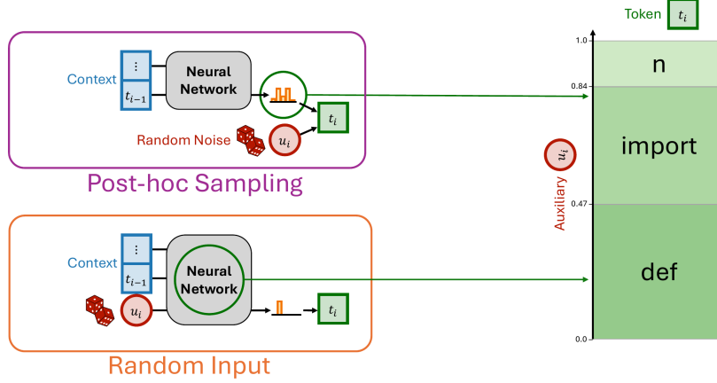
Figure 1: Moving the randomness. Top: standard decoding draws a distribution, then samples from it with auxiliary u_i . Bottom: PTP feeds u_i in as an input, so the token becomes a deterministic function of context and auxiliaries and future tokens become jointly predictable. Right: u_i selects a token by inverse CDF. Reproduced from the PTP framework (Draxler et al., 2025).
