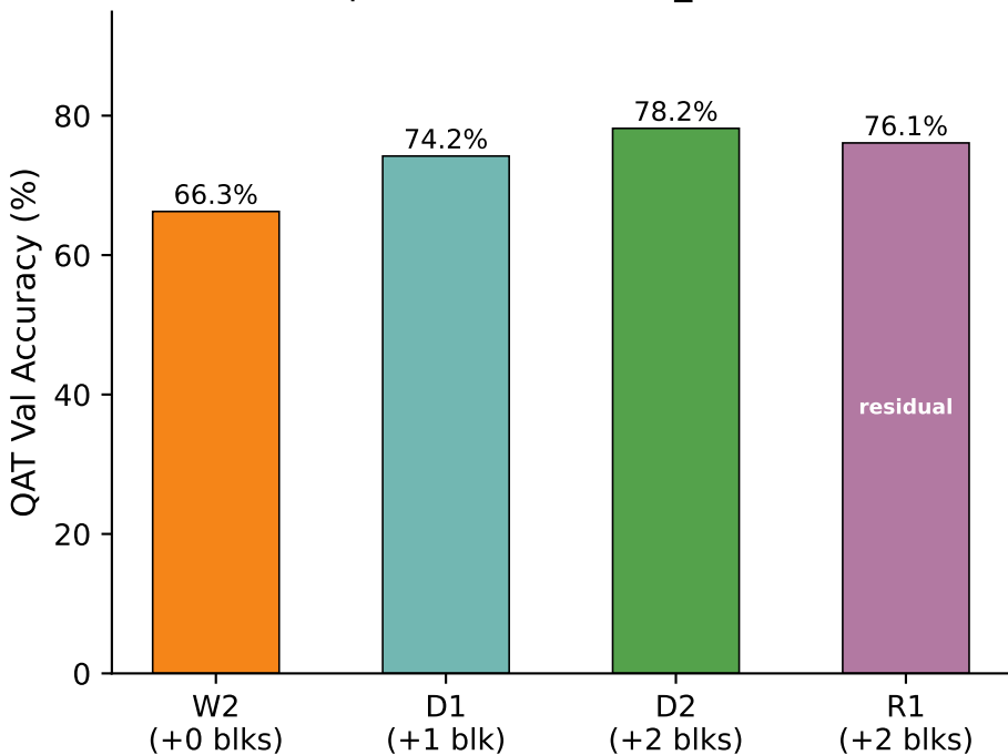
Depth Ablation (base_ch=16)
