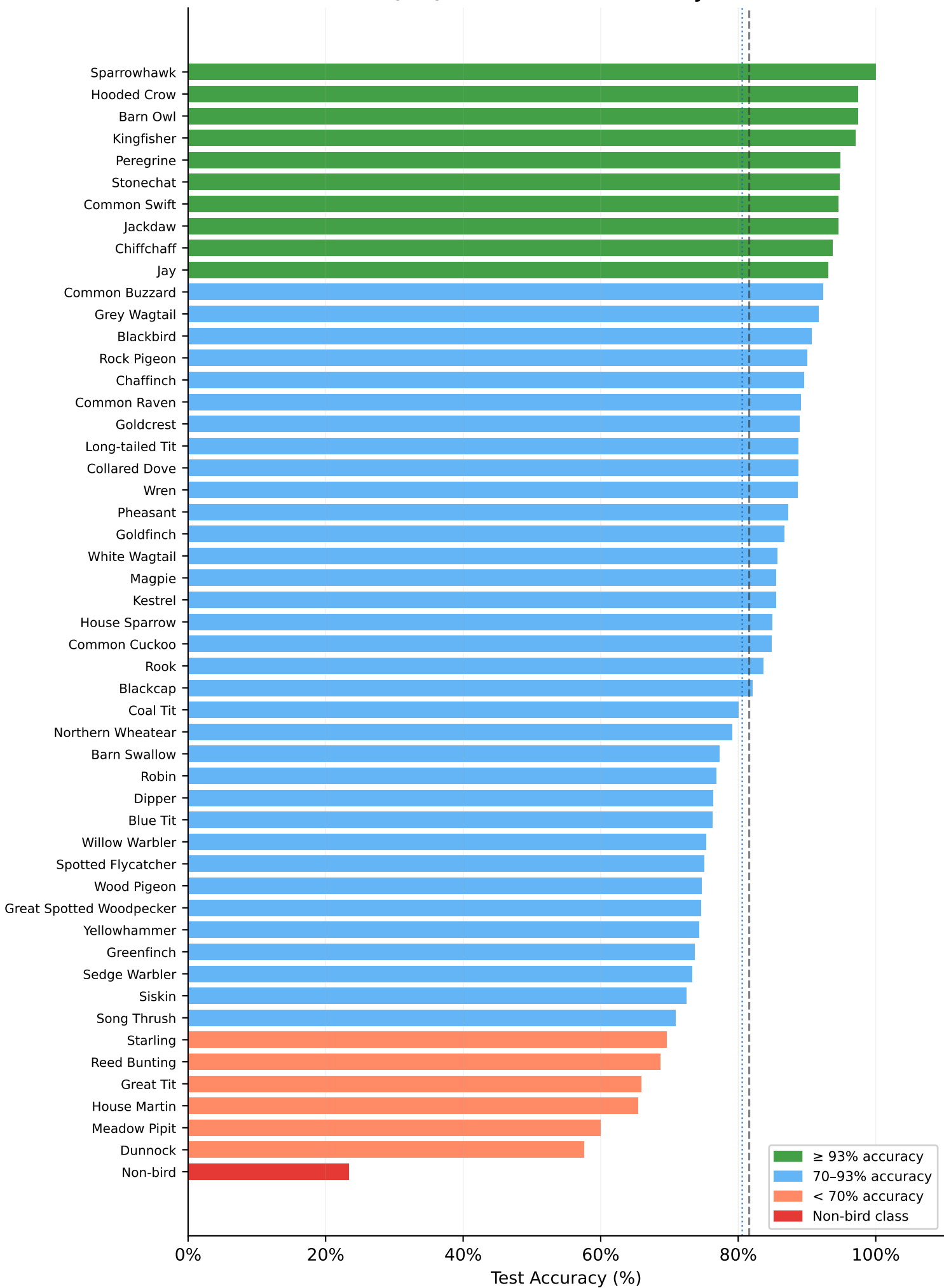
MicroBird (W3): Per-Class Test Accuracy — 51 Classes
