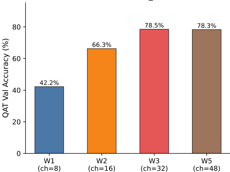
Width Ablation (extra_blocks=0)
