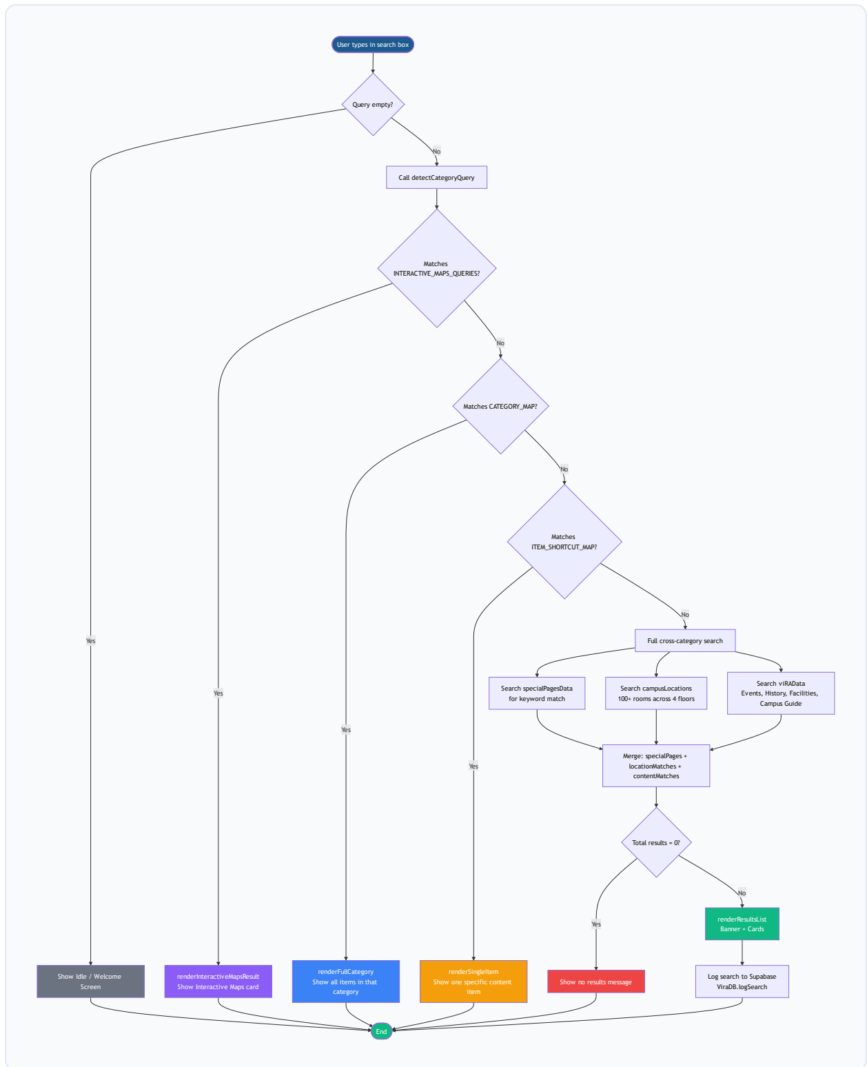
Diagram 6: 6. Activity Diagram — Search Flow
