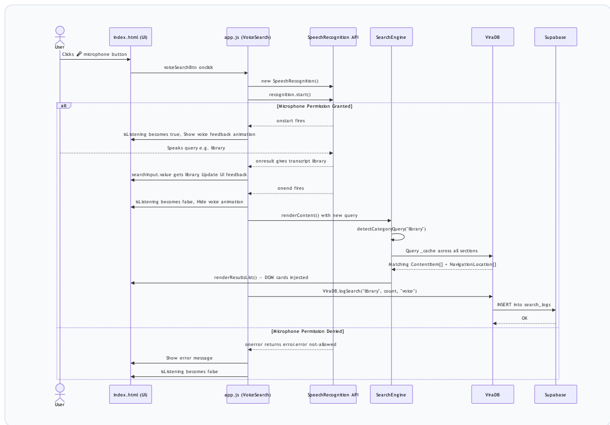
Diagram 4: 4. Sequence Diagram — Voice Search
