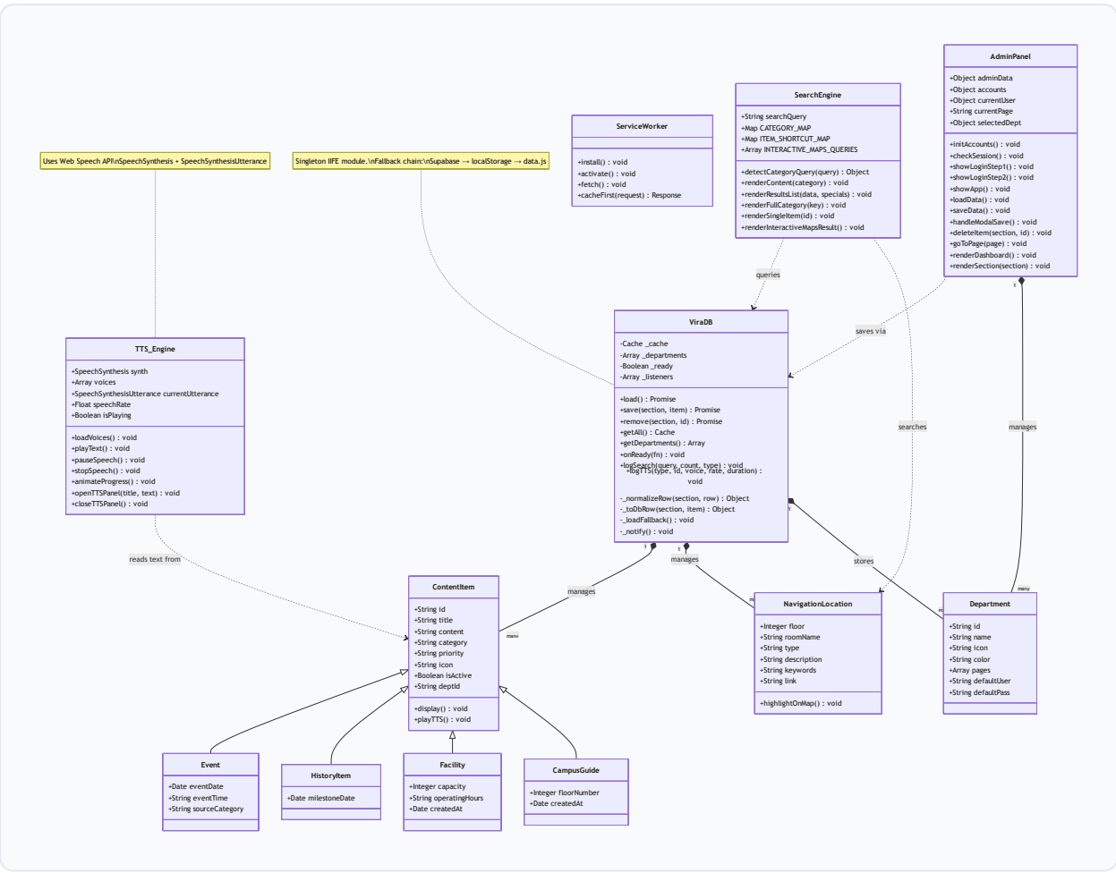
Diagram 2: 2. Class Diagram
