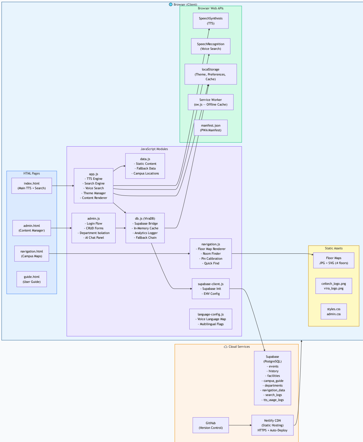
Diagram 8: 8. Component Diagram
