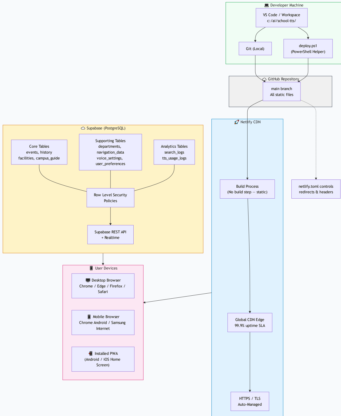
Diagram 9: 9. Deployment Diagram
