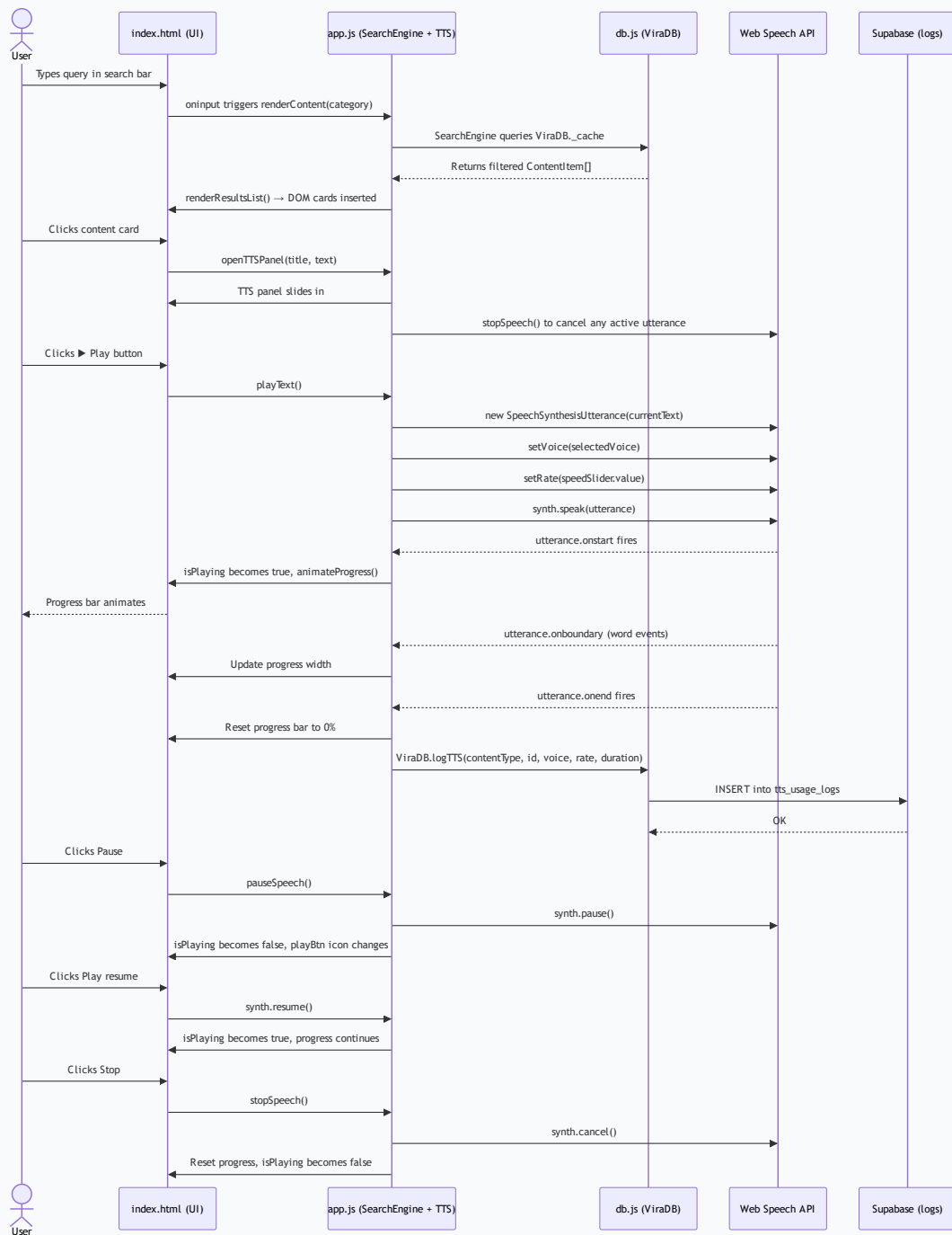
Diagram 3: 3. Sequence Diagram — TTS Playback
