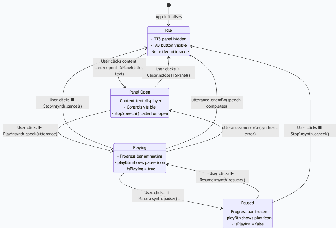
Diagram 7: 7. State Machine Diagram — TTS Player
