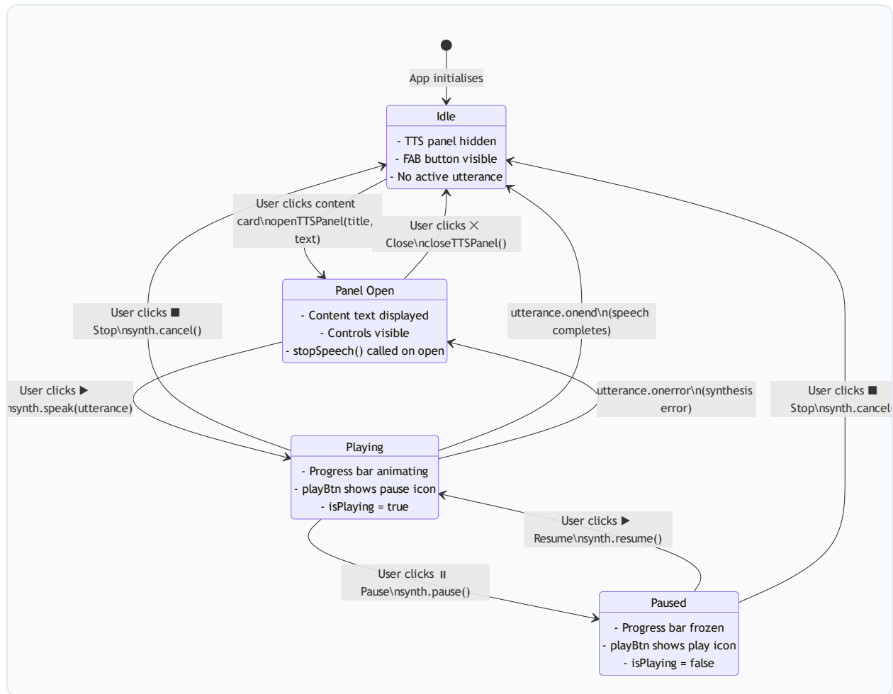
Diagram 7: 7. State Machine Diagram — TTS Player
