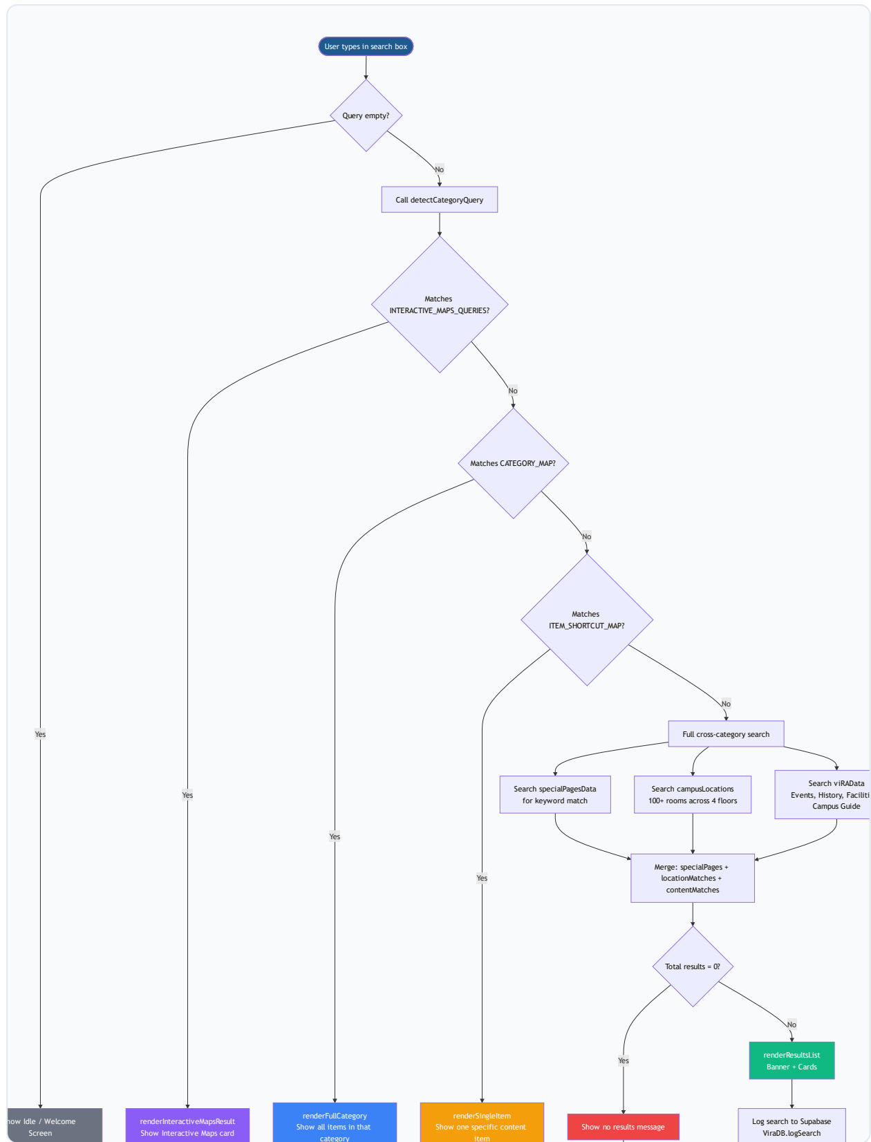
Diagram 6: 6. Activity Diagram — Search Flow
