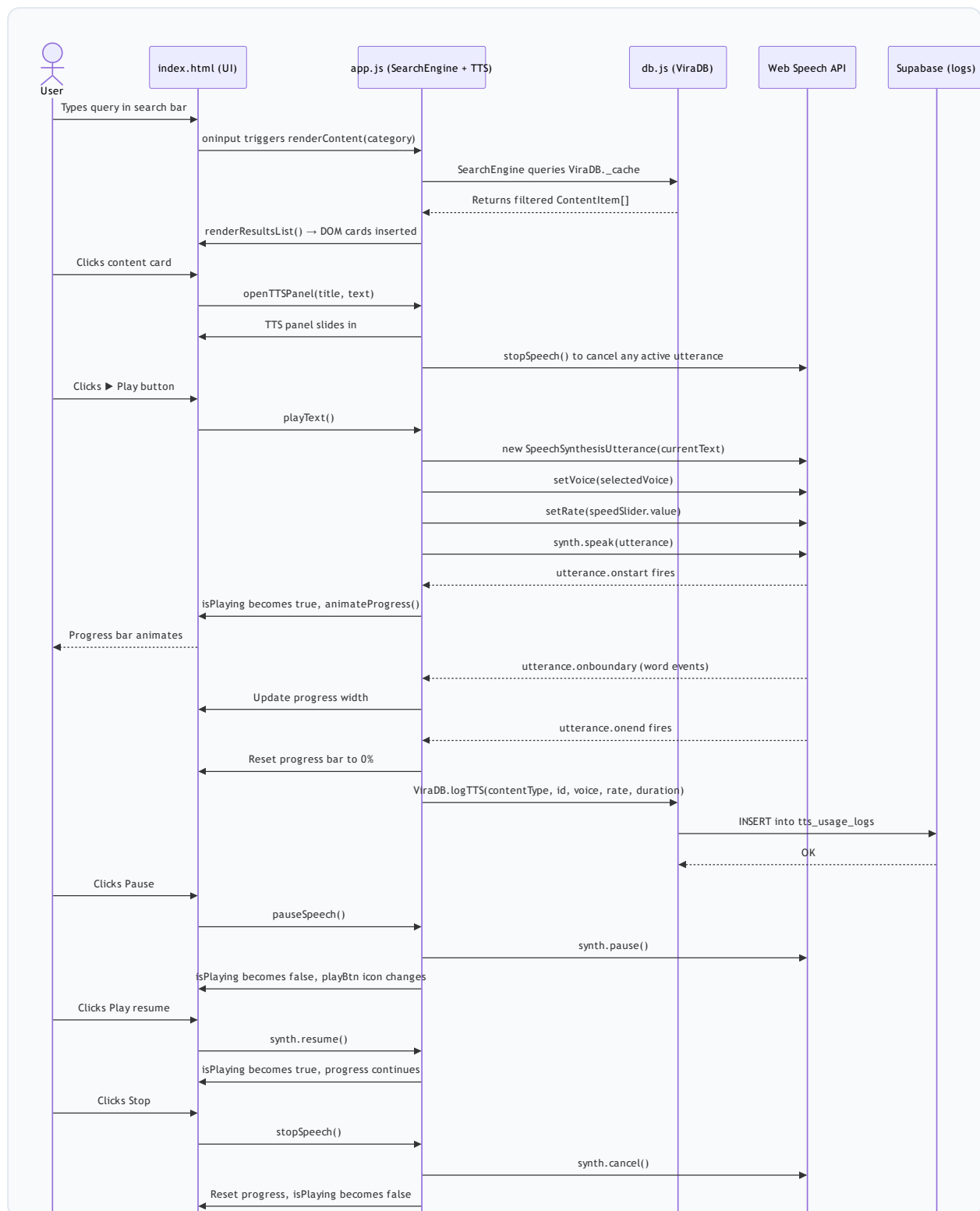
Diagram 3: 3. Sequence Diagram — TTS Playback
