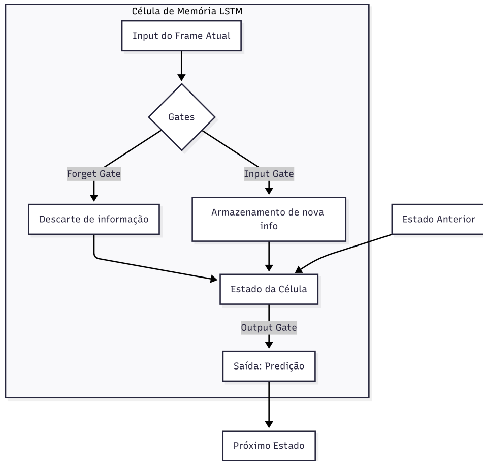
Figura 6 – Diagrama de Rede Neural LSTM.
