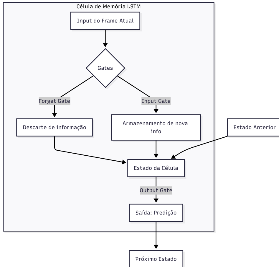
Figura 8 – Diagrama de Rede Neural LSTM.
