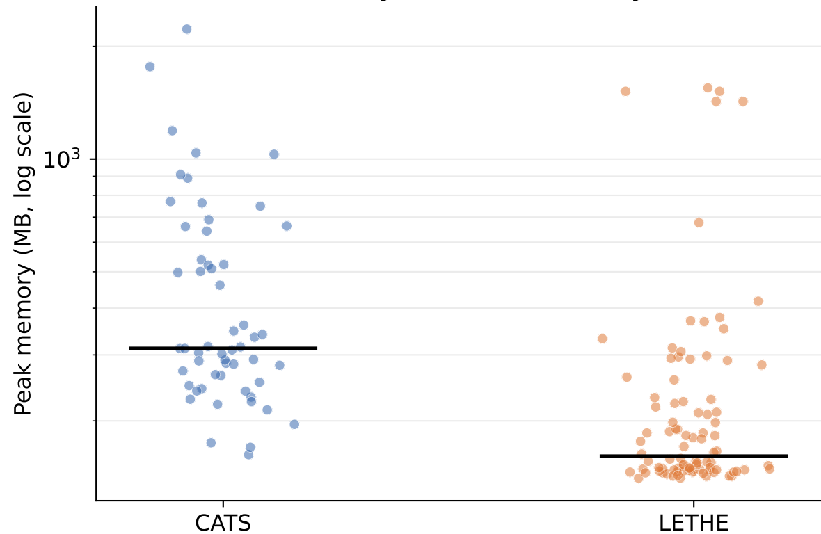
Peak memory of solved runs, by tool
