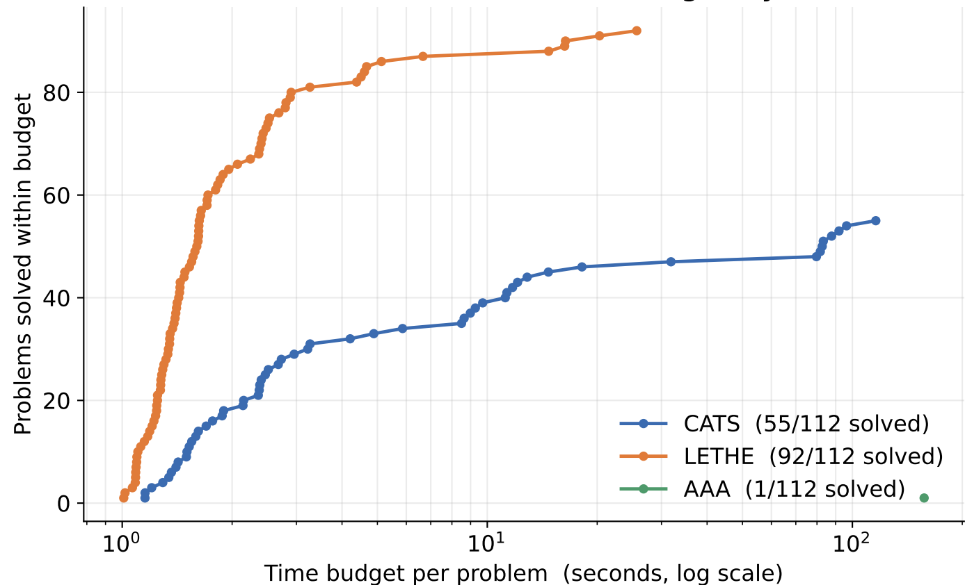
Problems solved within a time budget, by tool
