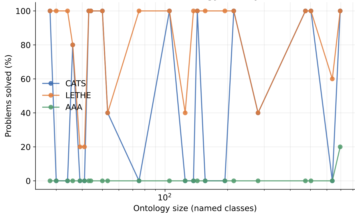
Solve rate vs ontology size, by tool
