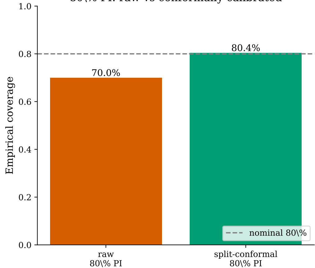
80\% PI: raw vs conformally calibrated
