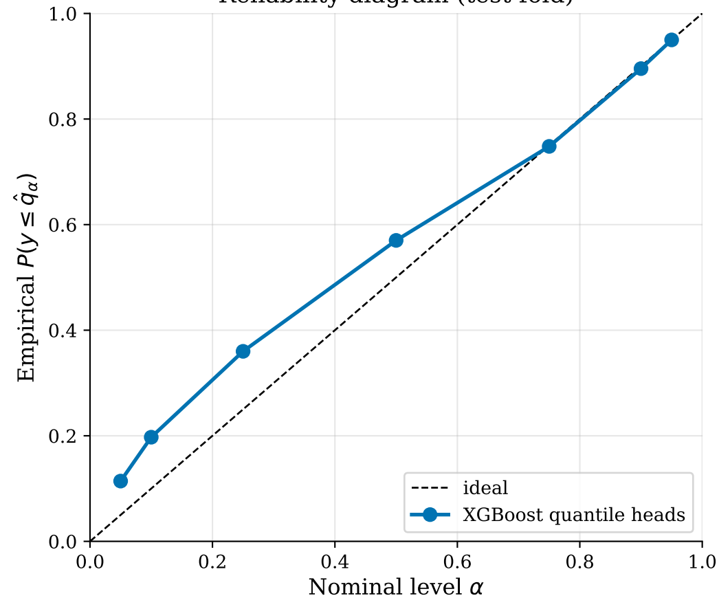
Reliability diagram (test fold)
