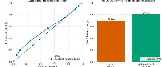
Figure 1: Left: reliability of the seven trained quantile heads on the test fold (predicted quantile \alpha vs. empirical P(y \leq \hat{q}_\alpha) ); the ideal line is y = x . Right: empirical coverage of the 80% PI before and after split-conformal calibration on the validation fold.
