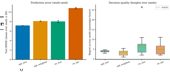
Figure 10: Left: mean test RMSE per method with one-SE error bars across 20 seeds. Right: boxplot of regret distributions across seeds (whiskers are 1.5 \times \text{IQR} ; dashed line at oracle). XGBoost-MSE has the lowest mean regret on this DGP; the decision-focused variants do not dominate it. The decision-weighted XGBoost has high RMSE but competitive regret. NN-MSE is unstable across seeds (outlier seeds inflate the box).
