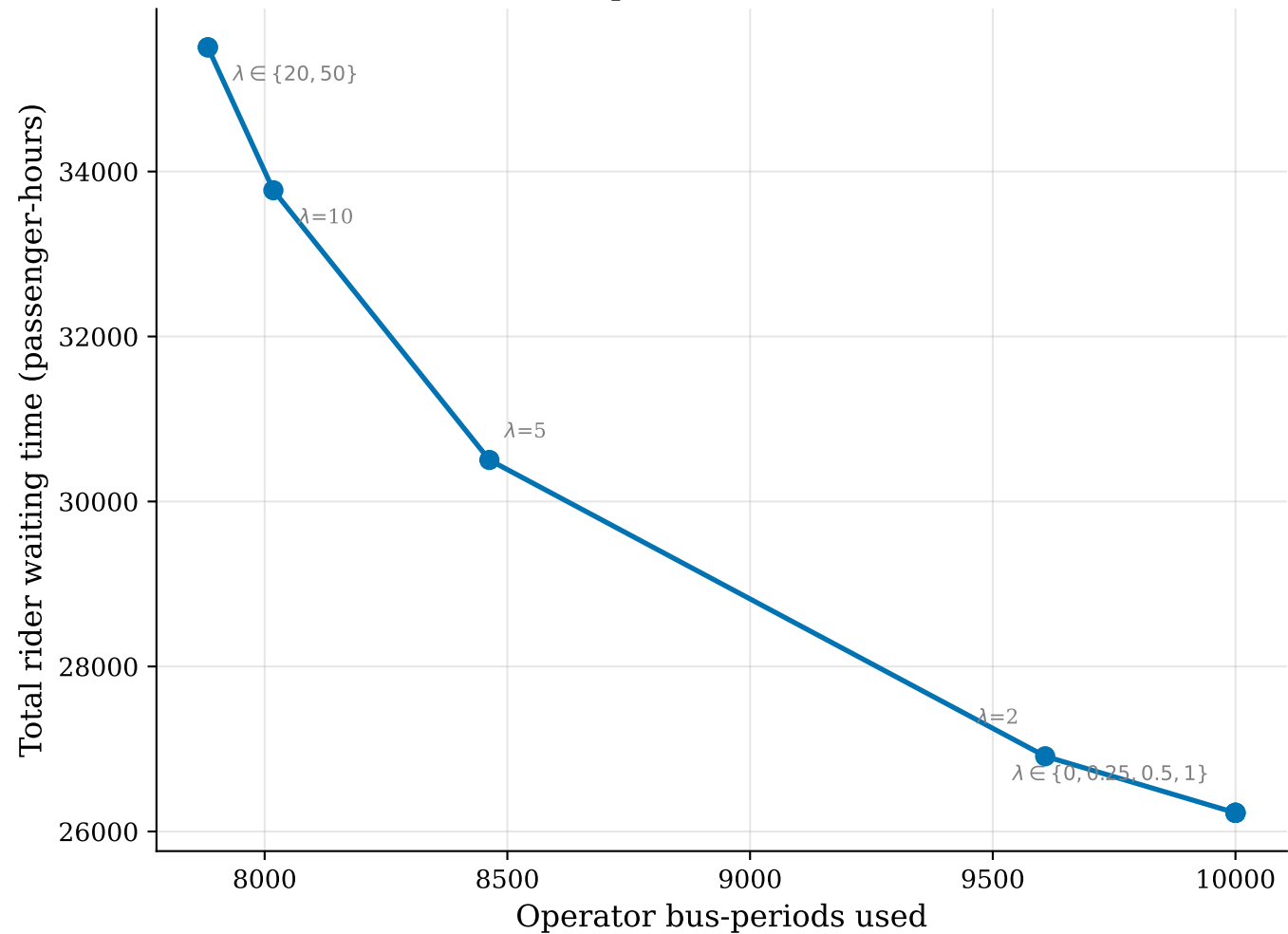
Rider wait vs operator cost: Pareto frontier
