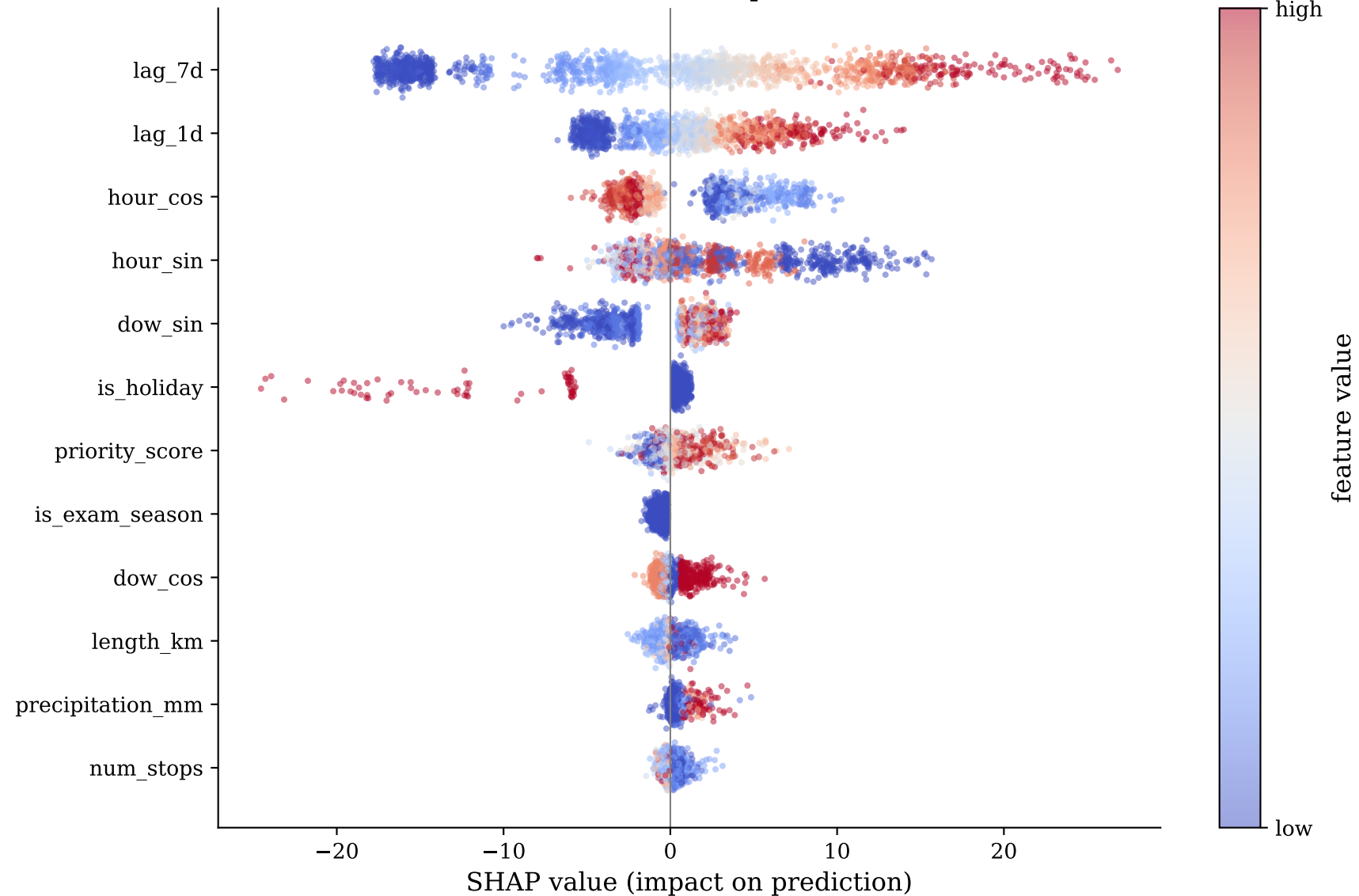
SHAP beeswarm — top 12 features
