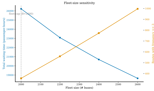
Figure 11: Fleet-size sensitivity. Left axis: total waiting time. Right axis: number of route-periods with frequency at least three. Vertical dashed line: peak-deployable fleet cap B = 2,000 (the status-quo schedule uses approximately 1,800 of these at peak).
