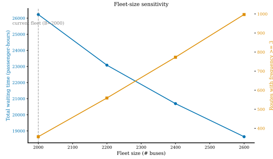
Figure 11: Fleet-size sensitivity. Left axis: total waiting time. Right axis: number of route-periods with frequency at least three. Vertical dashed line: current fleet B = 2,000 .
