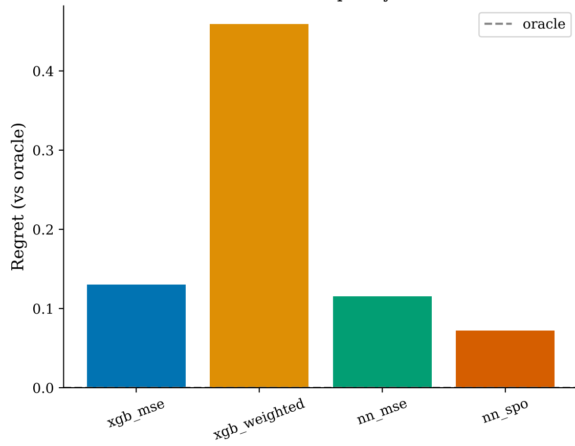
Decision quality
