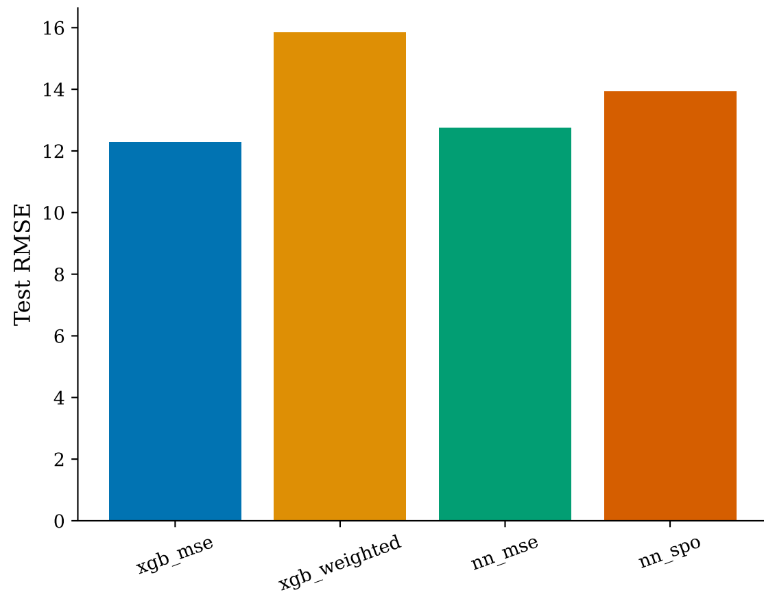
Prediction error
