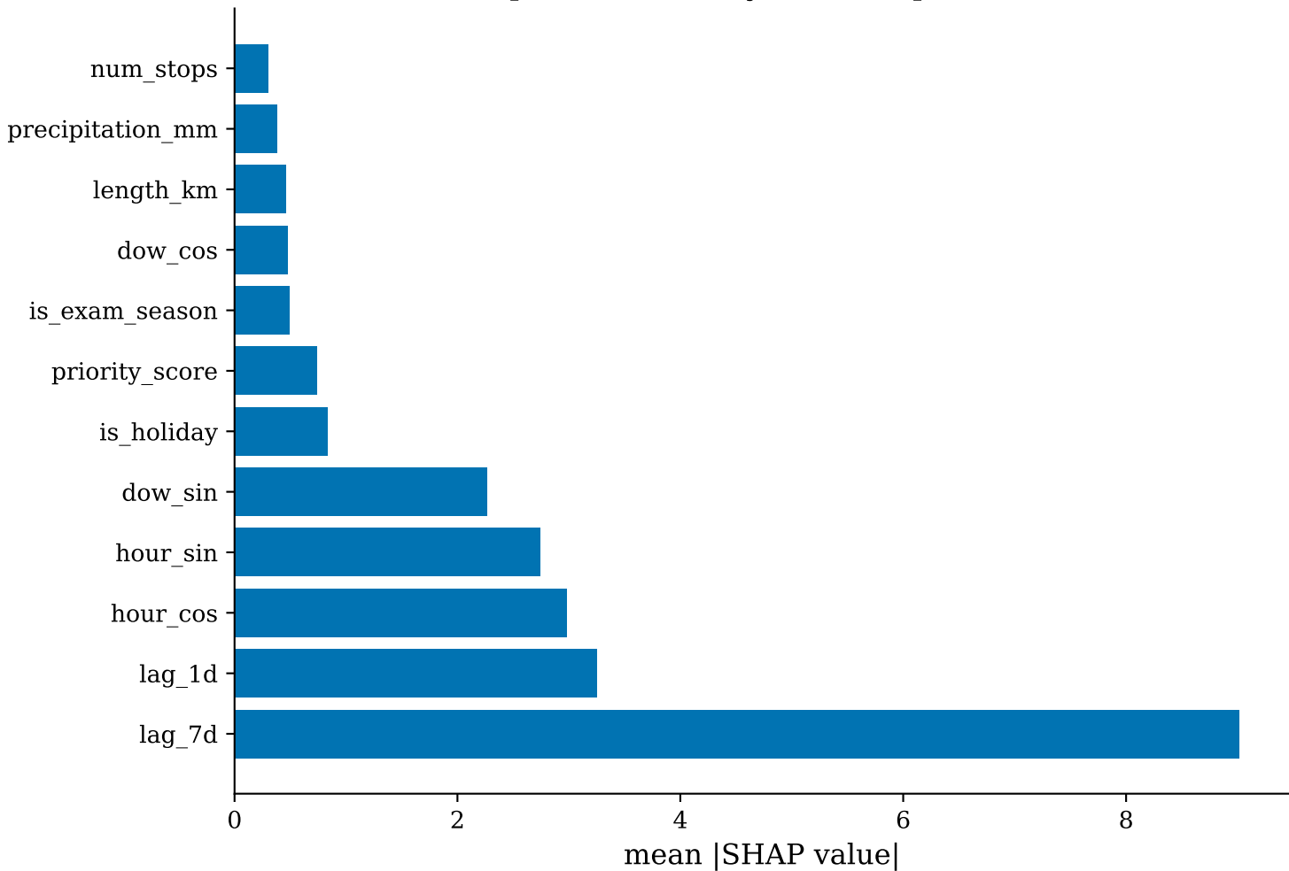
Top 12 features by SHAP importance
