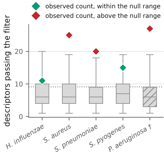
b: null range of the Route A1u hit count, 2.5th to 97.5th percentile of 1,000 permutations. Dotted line means 5 % of 182 tests, the naive expectation.
