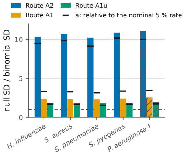
a: null SD of the hit count over the binomial SD of independent tests at the route's own null hit rate (bars) and at 5 % (ticks); dashed line: ratio = 1.
