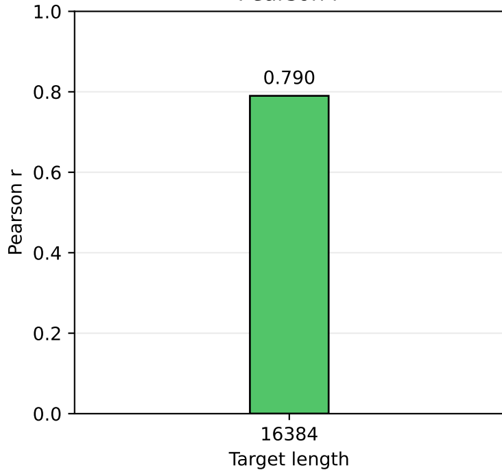
Pearson r
