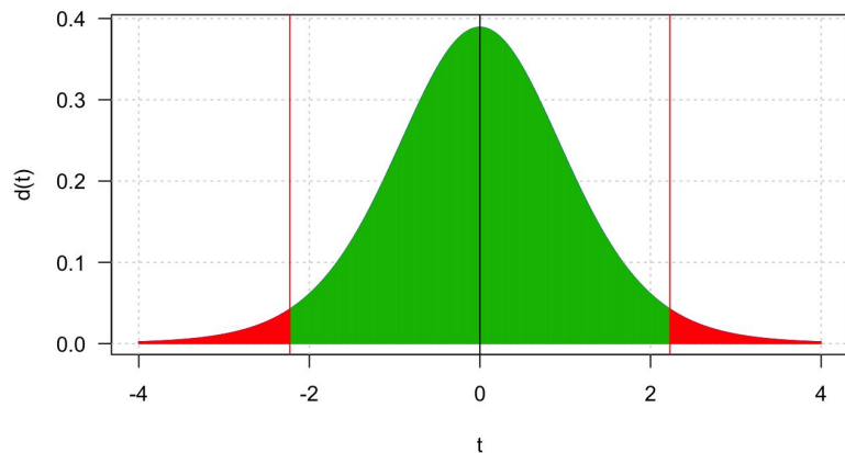
Student density, df=10
