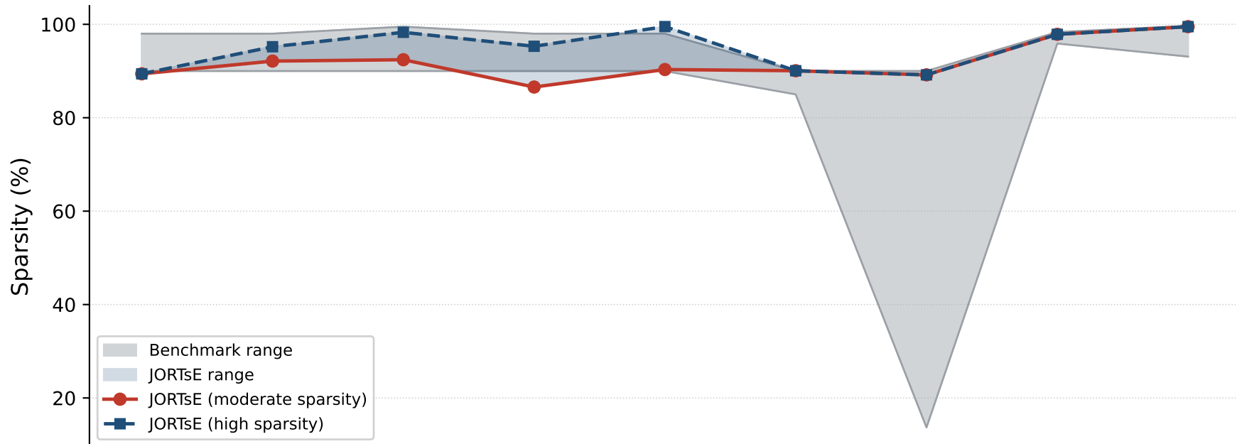
Sparsity
