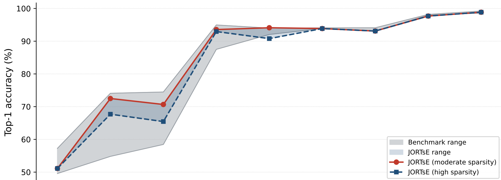
Accuracy
