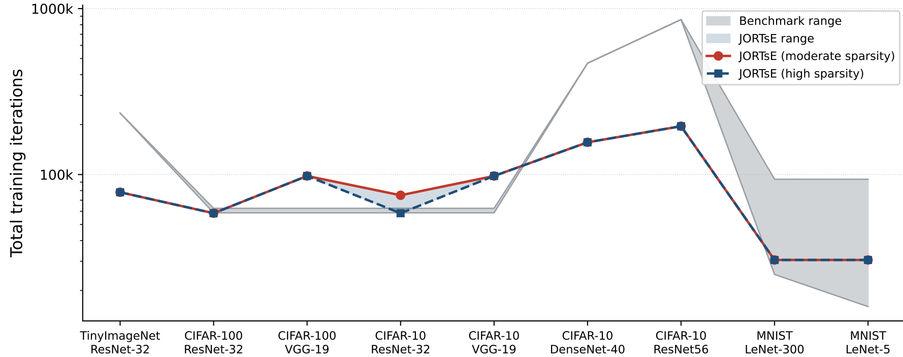
Training cost
