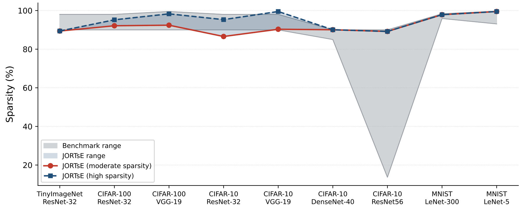
JORTsE vs Benchmarks: Sparsity
