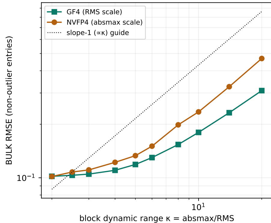
(A) synthetic: NVFP4 bulk error grows with \kappa
