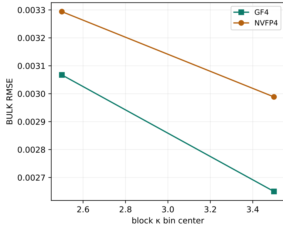
(C) real rotated fc2 acts: GF4 wins on high- \kappa blocks
