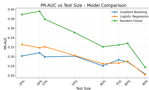
FIGURE 4.2: PR-AUC comparison for the baseline models
