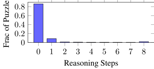
Figure 2. Halting distribution for halt-first ensemble (12 chains). 86.3% of puzzles have at least one chain halt at step 0; 94.9% within step 1.
