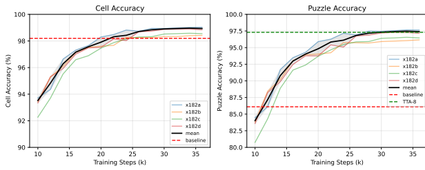
Figure 1. Learning curves across 4 seeds (fresh init). Left: Cell accuracy converges to 98.4–99.0%. Right: Puzzle accuracy reaches 96.2–97.6% by 36k steps. Fixed init shows identical final accuracy (96.9% ± 0.8%). Dashed lines: baseline (86.1%) and TTA-8 (97.3%).
