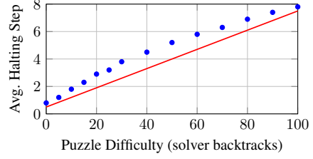
Figure 4. Halting step correlates with puzzle difficulty (measured by backtracking solver steps). Pearson r = 0.73 . The model takes longer on objectively harder puzzles.
