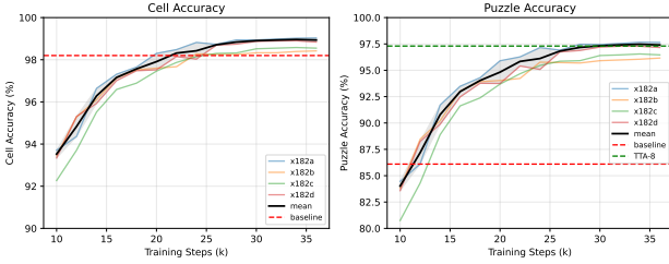
Figure 1. Learning curves across 4 seeds (random init variant). Left: Cell accuracy converges to 98.4–99.0%. Right: Puzzle accuracy reaches 96.2–97.6% by 36k steps. Learned init variant shows identical final accuracy (96.9% ± 0.8%). Dashed lines: baseline (86.1%) and TTA-8 (97.3%).
