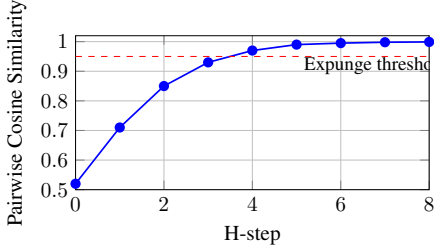
Figure 3. z_L convergence across heads during training. Pairwise cosine similarity exceeds 0.95 by step 4; expunging recovers compute for new samples.
