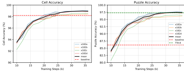
Figure 1: Learning curves across 4 seeds (fresh init). Left: Cell accuracy converges to 98.4–99.0%. Right: Puzzle accuracy reaches 96.2–97.6% by 36k steps. Fixed init shows identical final accuracy ( 96.9\% \pm 0.8\% ). Dashed lines: baseline (86.1%) and TTA-8 (97.3%).
