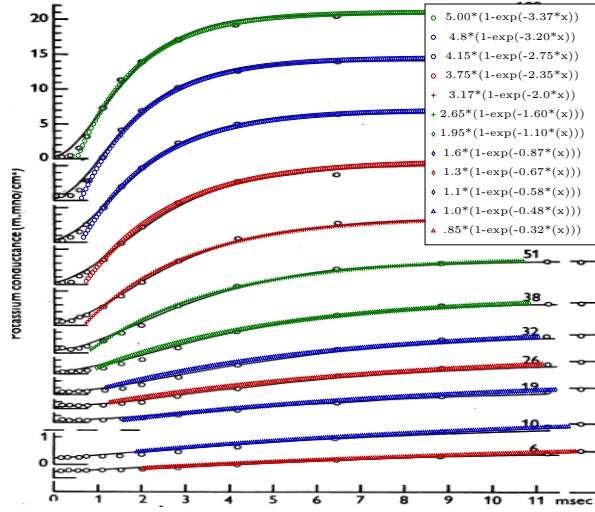
Figure 3.20: Finding time constants and membrane current by fitting data measured by HH (Fig. 3 in [13]) with our theoretically derived function (see Eq.(3.1)) (“Copyright [1991] Society for Neuroscience”)
