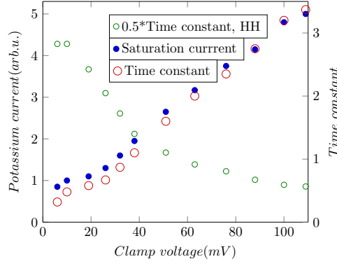
Figure 3.21: The experimental proof of the validity of the Stokes-Einstein relation to neurons. The proportionality of membrane's current (i.e., ions' speed) and time constant, respectively, with the clamping voltage (i.e., the voltage gradients). Data taken from Fig. 3.20 and Table I of [13], respectively.
