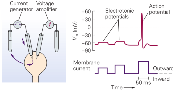
Figure 2.4: (Fig. 6.2c in [41]) Voltage recorded in presence of clamping current.
