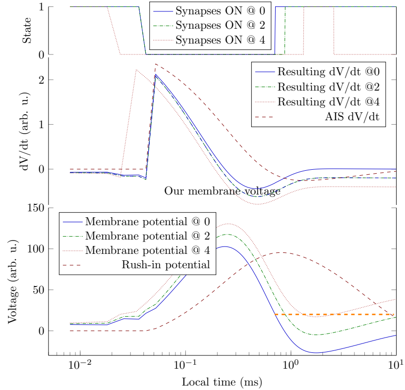
Figure 3.9: How the physical processes describe membrane's operation. The rushed-in Na^+ ions instantly increase the charge on the membrane, then the membrane's capacity discharges (produces an exponentially decaying voltage derivative). The ions are created at different positions on the membrane, so they need different times to reach the AIS, where the current produces a peaking voltage derivative. The resulting voltage derivative, the sum of the two derivatives, drives the oscillator. Its integration produces the membrane potential. When the membrane potential crosses the voltage threshold value, it switches the synaptic currents off/on.
