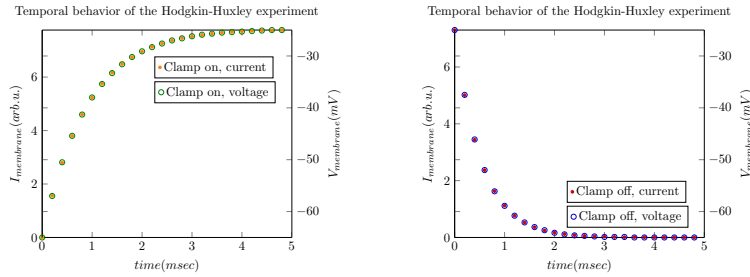
Figure 3.24: The time course of voltage and current a clamping experiment, calculated numerically for switching the clamping on and off.
