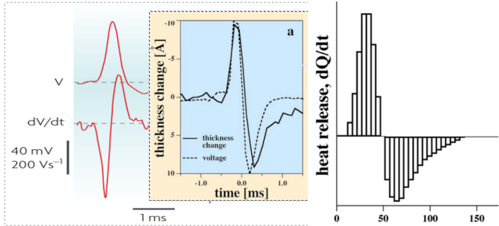
Figure 2.21: The time course of the electrical gradient [118] perfectly matches that of the mechanical and thermal changes [59]; however, classic theory cannot explain the connection between them [37]. The experimental \frac{dV}{dt} uses an opposite sign convention.
