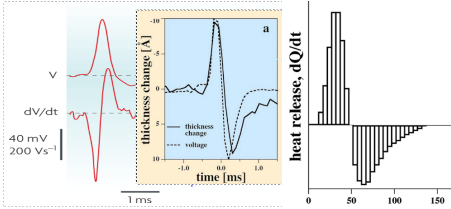
Figure 2.18: The red diagram lines show the membrane voltage and its gradient during producing an action potential [118], Fig. 4. The black diagram lines show the size-related and heat-related changes during producing an action potential [59], Fig. 1. and [94], Fig. 18.5. The voltage gradient has, by convention, opposite polarity.
