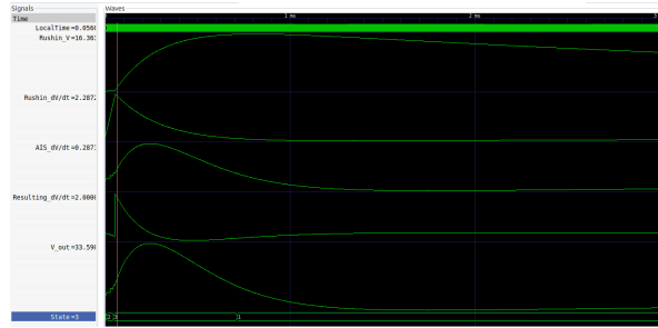
Figure 8.1: The summary of AP generation as seen in the simulator. The information is essentially the same that in Figure 3.15 (for codename '0', i.e., 'Simple delivery'). The rush-in current produces its voltage time derivative, the resulting voltage time derivative generates the neuron's output voltage, the AP. The neuron passes (due to the excitation) from stage 'Relaxing' (codename '1') to 'Computing' (codename '2') and 'Delivering' (codename '2') as described above.
