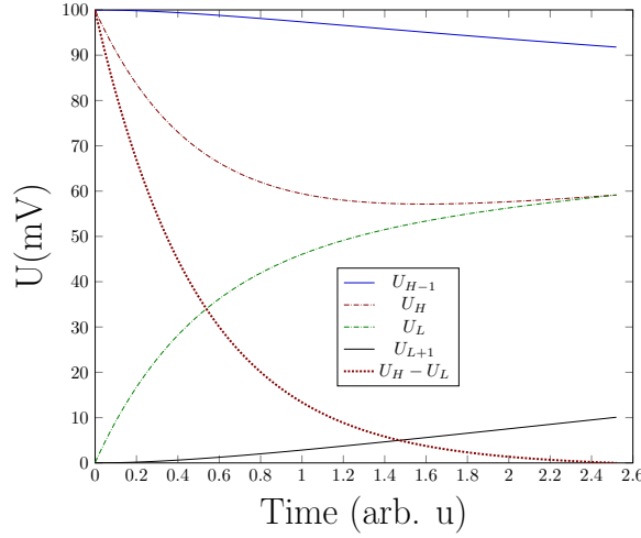
Figure 2.14: The potential values connected to the operation of ion channels. The arbitrary values of the transfer speeds (for visibility instead of approach real values) are \alpha = 1 ; \beta = .1 ; \gamma = 0.0001 ; furthermore the time scale is also arbitrary.
