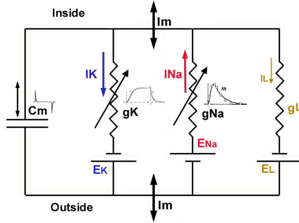
Figure 3.17: The equivalent circuit for the Hodgkin-Huxley model
