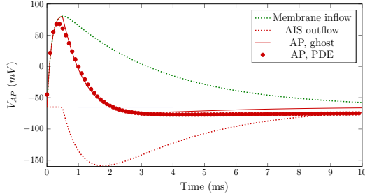
Figure 3.23: The "ghost image" formed by the delayed membrane current: the origin of the AP. The finite-speed ions transferred on the finite-size surface of the membrane: Kirchoff's Law in biology. The assumed delay time between input and output currents is 0.49 \text{ ms} , the function form and its parameters are displayed in Fig. 3.25.
