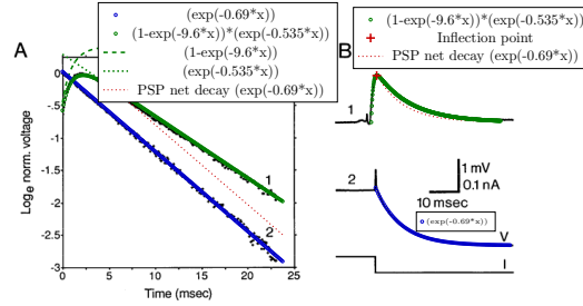
Figure 3.22: A) PSP decay (curve 1) and the decay after an injected depolarizing current pulse (curve 2) recorded in the same cell. B) Voltage traces (upper and middle) from which the curves in A were derived, together with the current record (lower) for the pulse. The colored marks and diagram lines are calculated using the model's "slow" current. Measurement data (with black) are reproduced from Fig. 4 of [85] ("©[1991] Society for Neuroscience").
