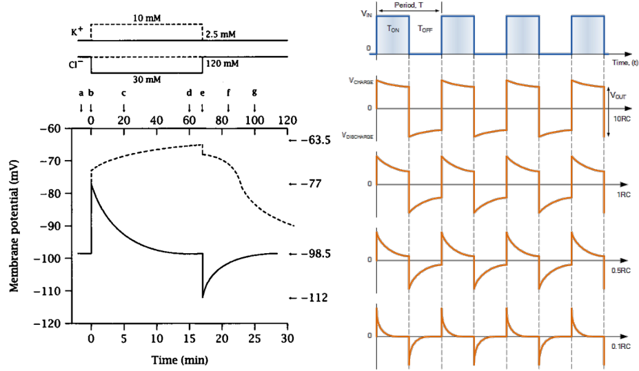
Figure 3.26: Left: The effect of applying a square-wave-like concentration change to membrane; Figure 2.2 from [2] Right: the effect of applying a square-wave like voltage change to an electric differentiator-type RC oscillator.
