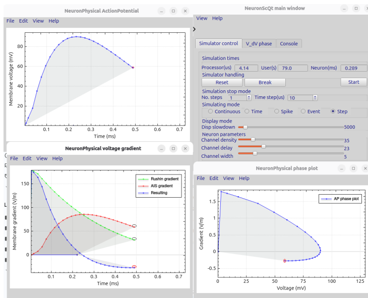
Figure 8.2: The ScQtNeuron simulator produces coordinated time diagrams about the neuron's electrical activity. The diagrams can be directly compared to experimentally measured ones. The control window enables to change the neuron's parameters.
