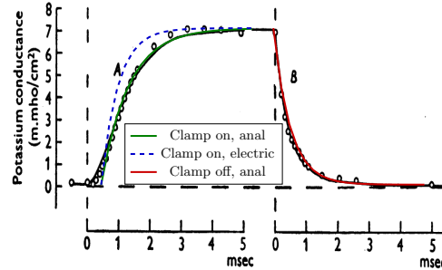
Figure 3.19: The green and red diagram lines are calculated for the clamping-on and clamping-off case. The dashed blue line models the case that the neuron is a purely electric system, as opposed to the case of clamping the axonal tube with ion channels in its wall. The black bulbs are for measured points. Moreover, the fitted polynomial line is reproduced from [13].
