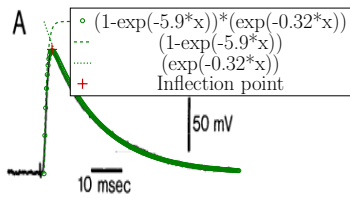
Figure 3.25: Time course of the post-synaptic potential evoked by a single AP. The colored marks and diagram lines are calculated using the model's "slow" current. Measurement data reproduced from Fig. 2 of [85] ("©[1991] Society for Neuroscience").
