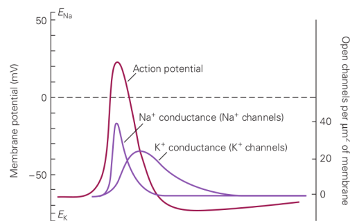
Figure 3.7: Errata in blue. (Fig. 7-1 in [41]). The sequential opening of voltage-gated Na^+ and K^+ channels generates the action potential. Wrong. The Na^+ channels are voltage controlled, and they open when AP is initiated. There are no K^+ channels in the game. Some resting K^+ channels exist and they contribute to the total current. Some K^+ flows out through the AIS, but it is by two order of magnitudes less then shown. Actually, these two currents are the condenser currents, before and after potential reversal on the condenser. The ' Na^+ current' is the current generated by the sharp 'switch-on' potential gradient, with a distortion caused by approxing the current's time course by a polynomial. One of Hodgkin and Huxley's great achievements was to dissect the change in conductance during an action potential into separate components attributable to the opening of Na^+ and K^+ channels. Mostly wrong. There is no change in conductance, it was a wong concept. They were tight in assuming the existence of ion channels and their opeing/closing, but it is not the case for Na^+ . The shape of the action potential and the underlying conductance changes can be calculated from the properties of the voltage-gated Na^+ and K^+ . Wrong. They used empirical measured distributions, instead of propertios of ion channels. (Adapted, with permission, from [13].)
