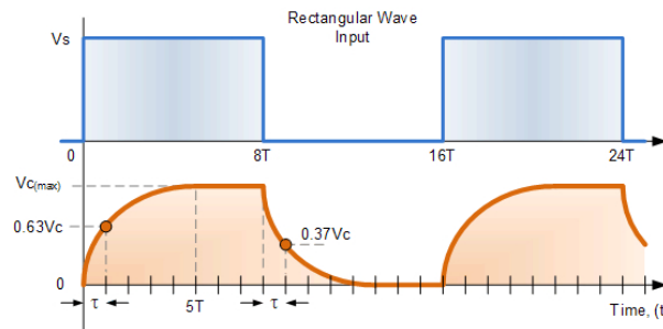
Figure 3.18: The output waveform of an integrator-type electric RC circuit at a long ( 8 * \tau ) pulse width square wave input (see Eq.( https://www.electronicstutorials.ws/ ))
