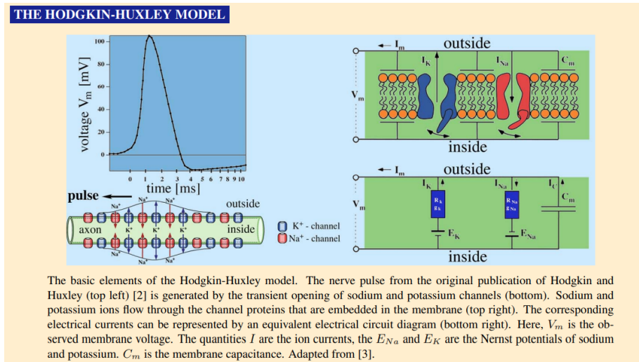
Figure 3.16: The Hodgkin-Huxley model as reproduced by [59]
