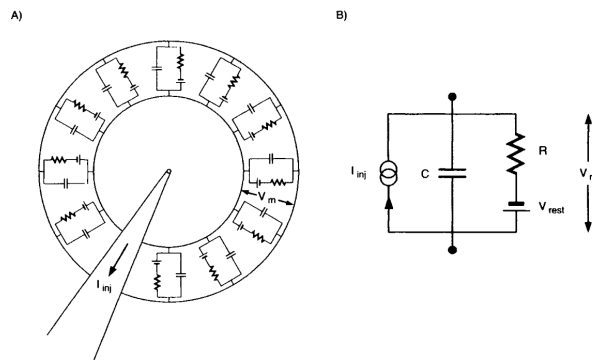
Figure 3.28: Equivalent electrical model of a spherical cell with passive membrane. [25] Fig. 1.2
