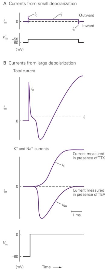
Figure 1.9: Errata in blue . A voltage-clamp experiment demonstrates the sequential activation of two types of voltage-gated channels. A. A small depolarization (10 mV) elicits capacitive and leakage currents ( I_c and I_l , respectively), the components of the total membrane current ( I_m ). There is no leakage current, see section 2.8.5 and the capacitive current is something different. The two small and opposite sharp changes are due to switching a current instead of voltage to the membrane (nothing is activated), see the signal shapes of the differentiator circle in Fig. 2.1. B. A larger depolarization (60 mV) results in larger capacitive and leakage currents, plus a time-dependent inward ionic current followed by a time-dependent outward ionic current. The larger current induces larger voltage gradient that opens voltage-controlled ion channels in the membrane's wall, and the slow current – distorted by the RC circuit as discussed– appears with a time delay on the the always-open channels in the AIS. Top: Total (net) current in response to the depolarization. Middle: Individual Na^+ and K^+ currents. Bottom: Voltage step and also current step . This is why I_c must be subtracted. I_K and I_{Na} are both capacitive currents, flowing in opposite directions, as discussed in section 2.4.6 (Fig. 7-3 in [41].)
