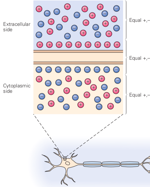
Figure 2.9: The cell membrane potential results from the separation of net positive and net negative charges on either side of the membrane. The excess of positive ions outside the membrane and negative ions inside the membrane represents a small fraction of the total number of ions inside and outside the cell at rest. (Fig. 6.1 in [41])
