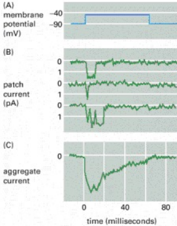
Figure 2.15: Patch-clamp measurements for a single voltage-gated Na^+ channel (Fig. 11.32 in [104]). Notice that due to the low current intensity, the measurement method comprises integration that "smears" line shape. Also notice that the shape of the aggregate current comprises different time contributions due to the different distances of channels from the measurement tip.
