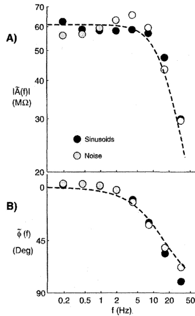
Figure 3.29: Illustrating the fallacy that neurons represent a low-pass filter. [25] Fig. 1.4
