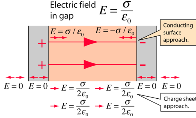
Figure 1.3: The oppositely charged parallel surfaces of the membrane are treated like conducting plates (infinite planes, neglecting fringing), then one can use Gauss's law to calculate the electrical field between the plates. Presuming the plates are at equilibrium with zero electrical fields inside the conductors, the result from a charged conducting surface can be used. "from Hyperphysics by Rod Nave, Georgia State University". © http://hyperphysics.phy-astr.gsu.edu/hbase/
