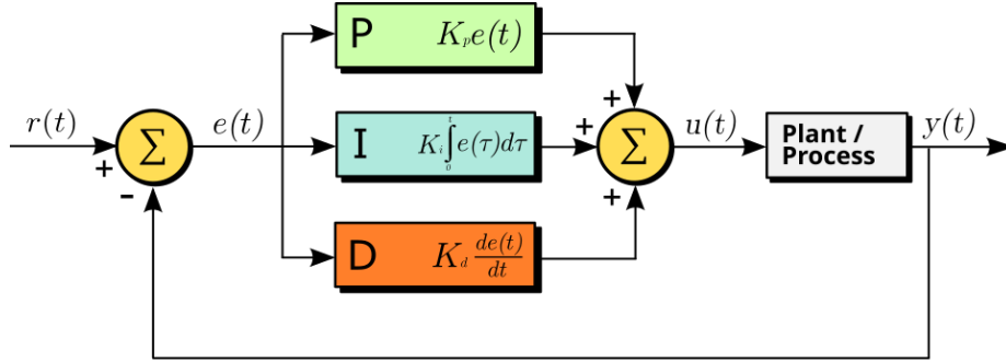
Figure 1.10: A block diagram of a PID controller in a feedback loop. r(t) is the desired process variable (PV) or setpoint (SP), and y(t) is the measured PV. (Wikipedia)
