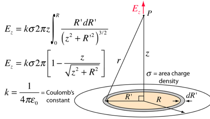
Figure 1.2: The electrical field of a disc of charge can be found by superposing the point charge fields of infinitesimal charge elements. This field can be facilitated by summing the fields of charged rings. “From Hyperphysics by Rod Nave, Georgia State University”. ©hyperphysics.phy-astr.gsu.edu/hbase/
