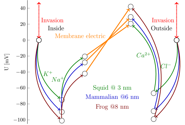
Figure 1.8: The mechanism for controlling neuronal operation is the same in all cases shown in Table 1.1. It appears that the thicker membrane produces a higher membrane electrical potential, requiring a higher thermal potential to compensate. However, it can solve the task using a lower salt concentration, since the electrical membrane potential accelerates ion flow through the membrane channels, thereby speeding up the operation. The electrical fields for the different species have similar values, as shown in Fig. 1.1. Furthermore, the total concentration decreases as the membrane thickness and potential increase.
