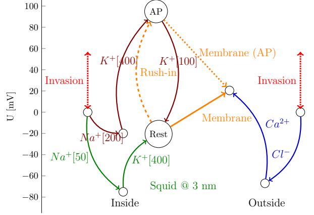
Figure 1.9: The mechanism of producing AP (using numbers referring to the case of squid shown in Table 1.1). In the resting state, the inside thermal potentials follow the green paths. When the rush-in of Na^+ ions suddenly increases the internal concentration to [200], the potential on the internal side of the membrane increases to +90 mV. The neuron must decrease its concentrations to restore the resting potential, mainly by releasing an action potential through the AIS.
