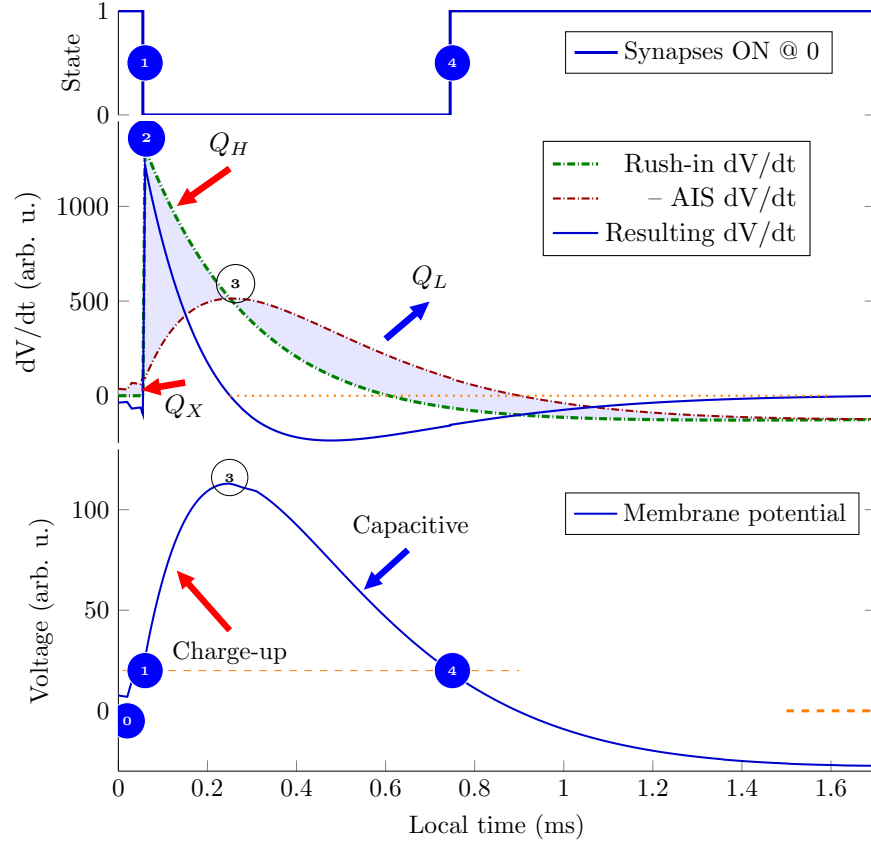
Figure 1.12: The physical processes describing the membrane's operation. The rush-in Na^+ ions instantly increase the membrane's charge, and the membrane's capacity discharges (producing an exponentially decaying voltage derivative). The ions are created at different positions on the membrane, so they take different times to reach the AIS, where the current produces a peak in the voltage derivative. The resulting voltage derivative, the sum of the two derivatives (the AIS current is outward), drives the oscillator. Its integration produces the membrane potential. When the membrane potential crosses the threshold, it switches the synaptic currents on or off.
