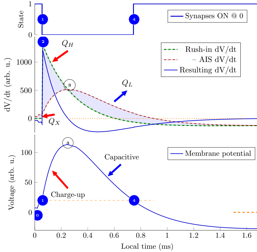
Figure 2.19: The physical processes describing the membrane's operation. The rush-in Na^+ ions instantly increase the membrane's charge, and the membrane's capacity discharges (producing an exponentially decaying voltage derivative). The ions are created at different positions on the membrane, so they take different times to reach the AIS, where the current produces a peak in the voltage derivative. The resulting voltage derivative, the sum of the two derivatives (the AIS current is outward), drives the oscillator. Its integration produces the membrane potential. When the membrane potential crosses the threshold, it switches the synaptic currents on or off.
