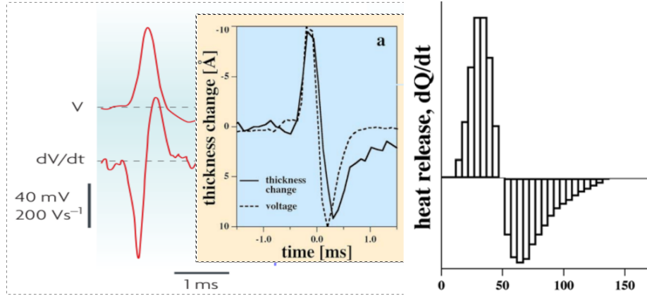
Figure 2.18: The red diagram lines show the membrane voltage and its gradient during producing an action potential [118], Fig. 4. The black diagram lines show the size-related and heat-related changes during producing an action potential [59], Fig. 1. and [94], Fig. 18.5. The voltage gradient has, by convention, opposite polarity.
