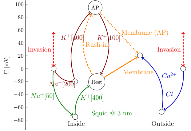
Figure 6.9: The mechanism of producing AP (using numbers referring to the case of squid shown in Table 6.1). In the resting state, the inside thermal potentials follow the green paths. When the rush-in of Na^+ ions suddenly increases the internal concentration to [200], the potential on the internal side of the membrane increases to +90 mV. The neuron must decrease its concentrations to restore the resting potential, mainly by releasing an action potential through the AIS.
