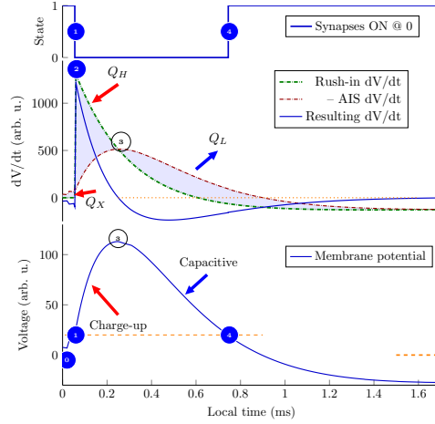
Figure 1.7: The summary of AP generation. The voltage time derivatives (the middle inset), resulting by summing the \frac{d}{dt}V_{AIS} , \frac{d}{dt}V_M and a constant corresponding to the clamping current, that define the membrane's output voltage (the AP, the bottom subfigure), that control synaptic contributions (top subfigure).
