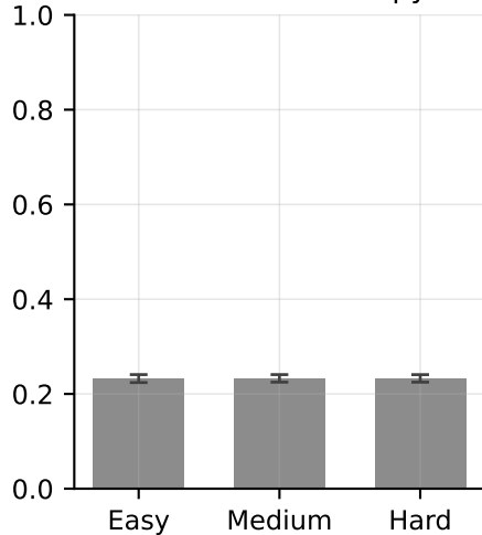
1: Attention entropy
