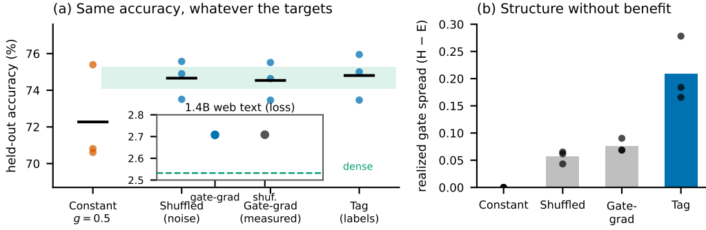
Figure 2: The content-irrelevance punchline, both scales. (a) 11M Stage-2 arms at an identical inference budget ( \sim 19 MFLOPs/token; the oracle pass is billed to both measured arms); dots are individual seeds, all arms forking from the same Stage-1 body per seed. True-label, measured-value, and noise targets land in one green tie band (max paired difference 0.3 points); a constant gate in the same protocol sits 2.4 points below. Inset : the 1.4B replication, gate-grad vs. shuffled held loss ( |\Delta| = 0.0008 ; the 1.0-point rule was pre-registered in accuracy at 11M and has no NL loss-domain twin; the two dots sit at nearly the same height). (b) Realized hard-minus-easy gate spread: only the tag arm builds difficulty-ordered gates ( r = 0.95 ), structure without accuracy benefit. Numbers: Table 4 (Appendix C).
