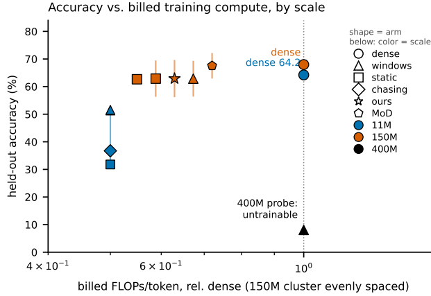
Figure 3: Accuracy vs. billed training compute (relative to the dense arm at the same scale, log axis; marker = arm, color = scale, values in Tables 1 and 2. The five gated 150M arms share a 0.57–0.59 \times budget, so their x positions are evenly spaced for readability rather than to scale). Gated 2-stage arms cluster at \sim 0.58\times dense compute and \sim 5 points below it at 150M; MoD reaches dense compute savings with an inverted router. The 400M probe collapses (post-LN + Xavier init, untrainable at the preset per-size LRs tried), the honest edge of the scaling evidence; 1B was never run.
