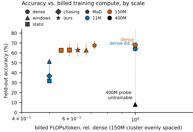
Figure 3: Accuracy vs. billed training compute (relative to the dense arm at the same scale, log axis; marker = arm, color = scale, values in Tables 1 and 2. The five gated 150M arms share a 0.57–0.59 \times budget, so their x positions are evenly spaced for readability rather than to scale). Gated 2-stage arms cluster at \sim 0.58\times dense compute and \sim 5 points below it at 150M; MoD reaches dense compute savings with an inverted router. The 400M probe collapses (post-LN + Xavier init, untrainable at the preset per-size LRs tried), the honest edge of the scaling evidence; 1B was never run.
