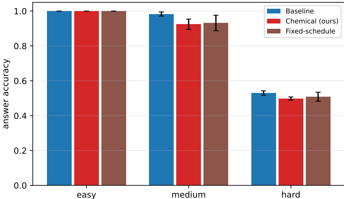
Per-difficulty accuracy (tagged)
