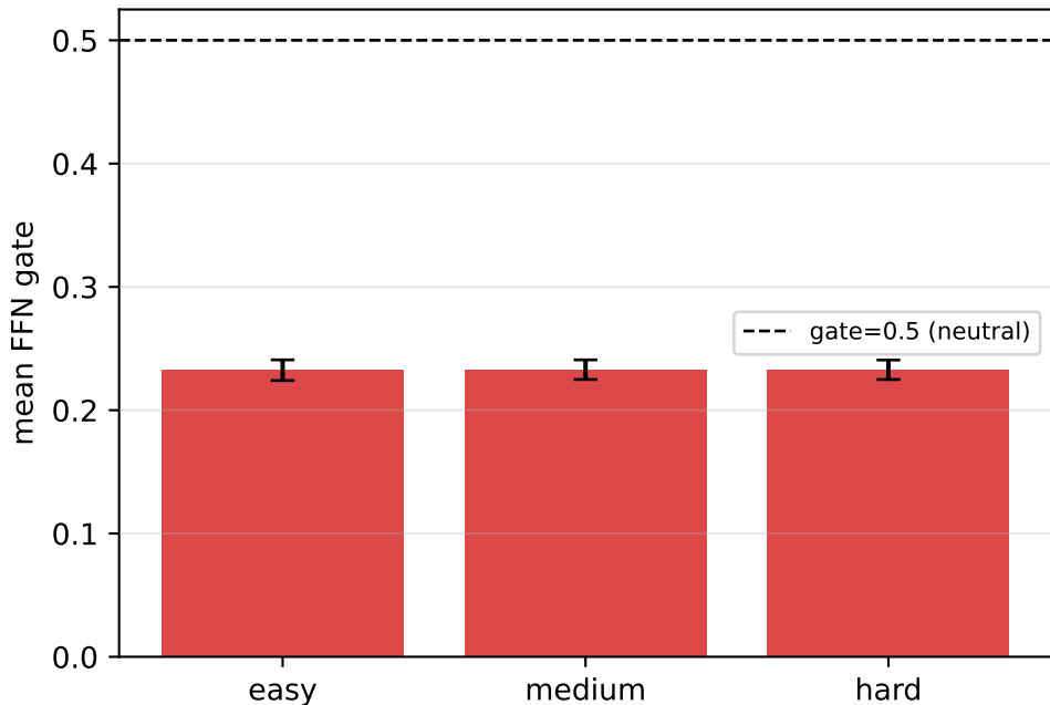
Mean FFN gate by difficulty (tagged)
