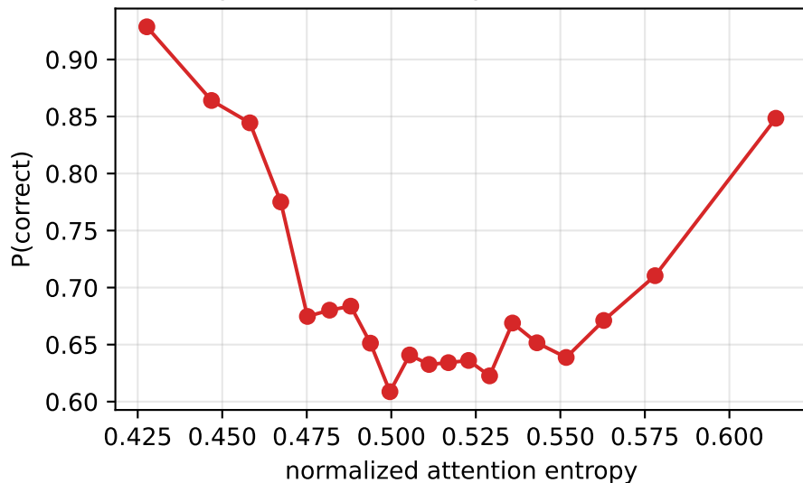
Entropy vs correctness (tagged) pearson -0.067, spearman -0.089
