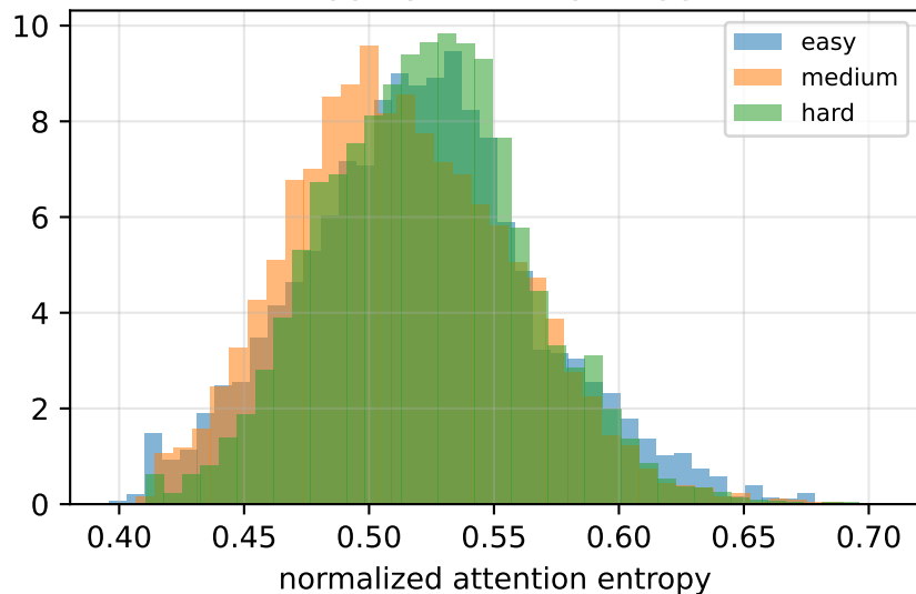
Entropy by difficulty (tagged)
