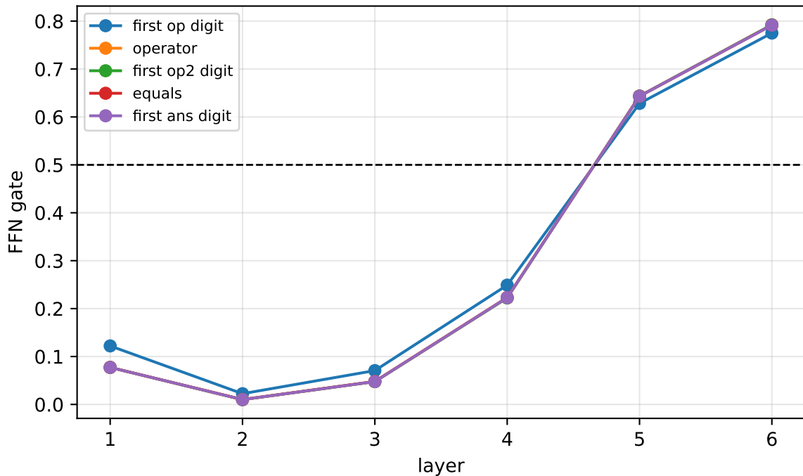
Layer-wise gate trajectory: 4-digit multiplication (mixed)
