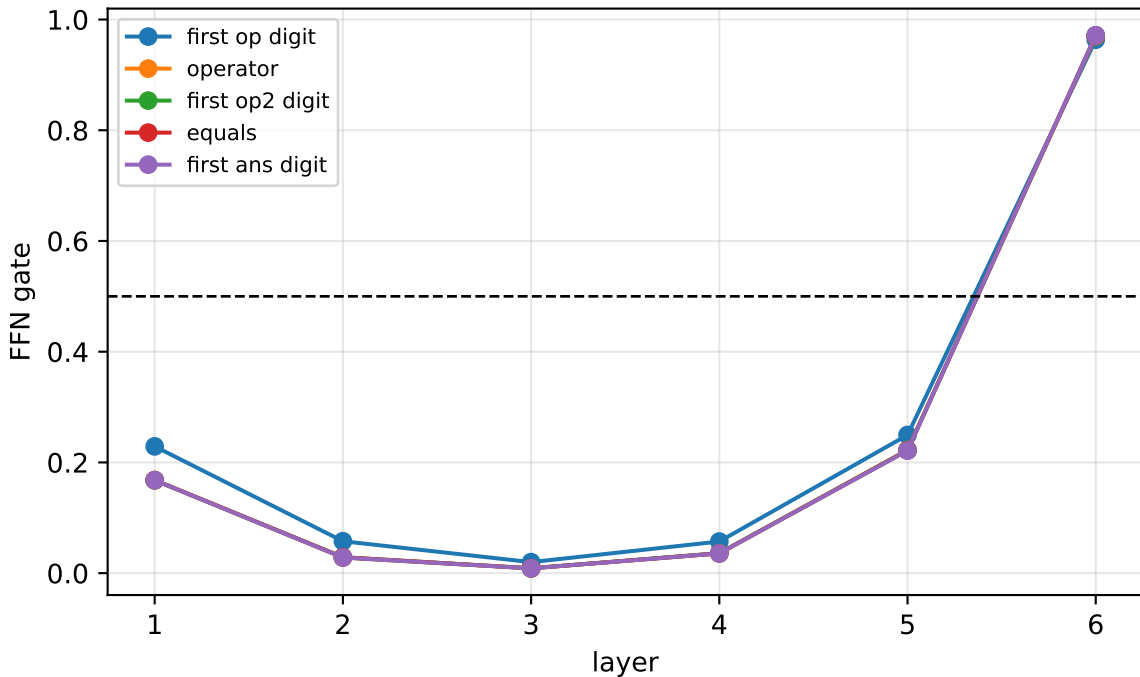
Layer-wise gate trajectory: hard multiplication (tagged)
