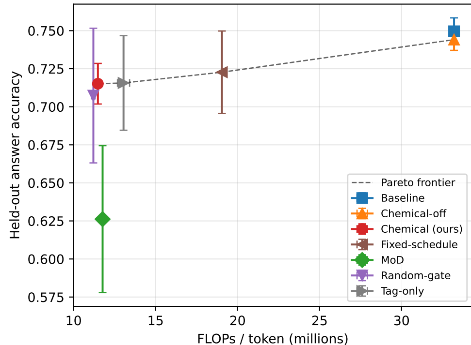
tagged arithmetic
