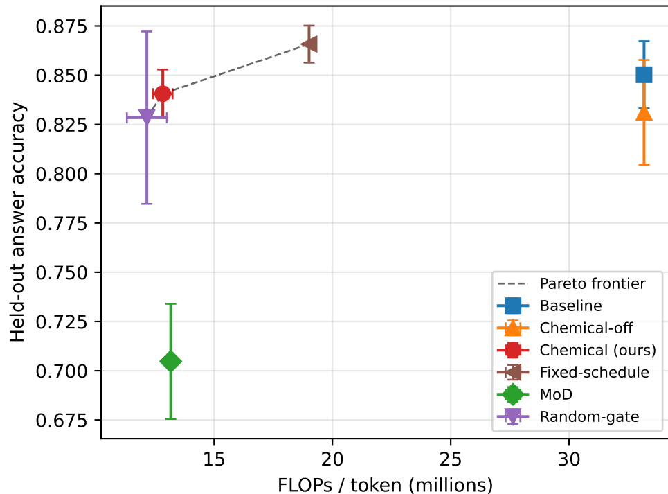
mixed arithmetic
